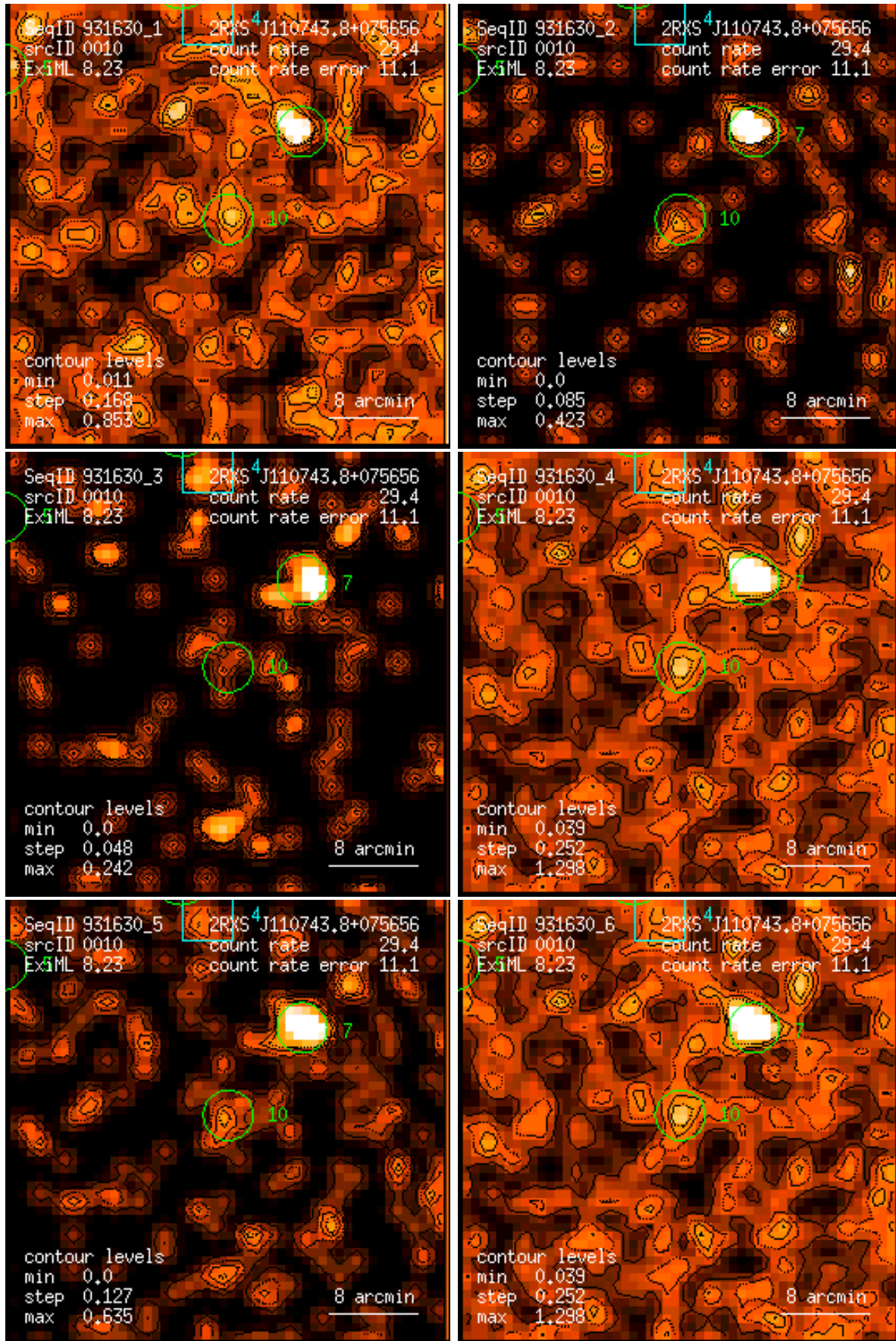
Figure 10: RASS 931630: detection 0010: band rate images, Gaussian filter: (1) PSPC channels 11 – 41, (2) 52 – 90, (3) 91 – 201, (4) 11 – 235, (5) 52 – 201, (6) 11 – 201. Broad band rates in counts/ks. Band rate contour levels in counts/ks/arcmin 2 .
