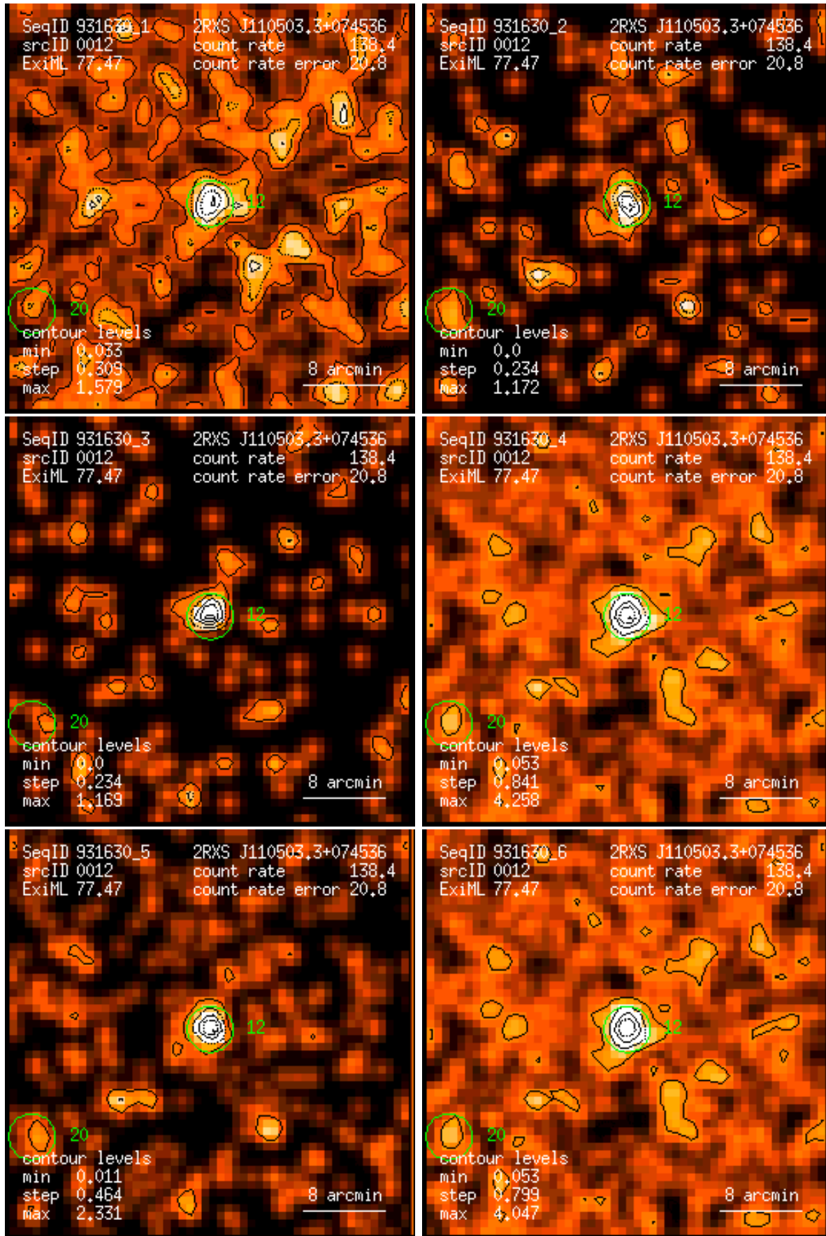
Figure 12: RASS 931630: detection 0012: band rate images, Gaussian filter: (1) PSPC channels 11 – 41, (2) 52 – 90, (3) 91 – 201, (4) 11 – 235, (5) 52 – 201, (6) 11 – 201. Broad band rates in counts/ks. Band rate contour levels in counts/ks/arcmin 2 .
