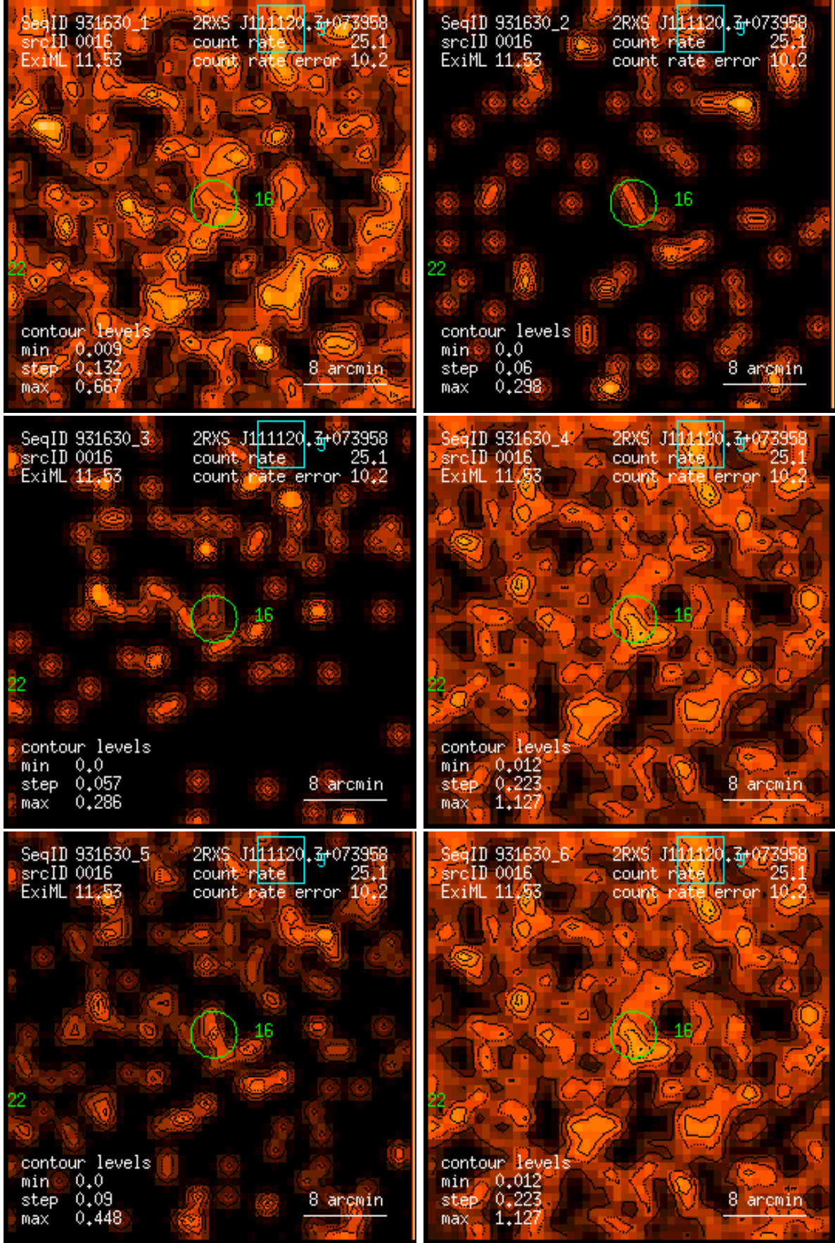
Figure 16: RASS 931630: detection 0016: band rate images, Gaussian filter: (1) PSPC channels 11 – 41, (2) 52 – 90, (3) 91 – 201, (4) 11 – 235, (5) 52 – 201, (6) 11 – 201. Broad band rates in counts/ks. Band rate contour levels in counts/ks/arcmin 2 .
