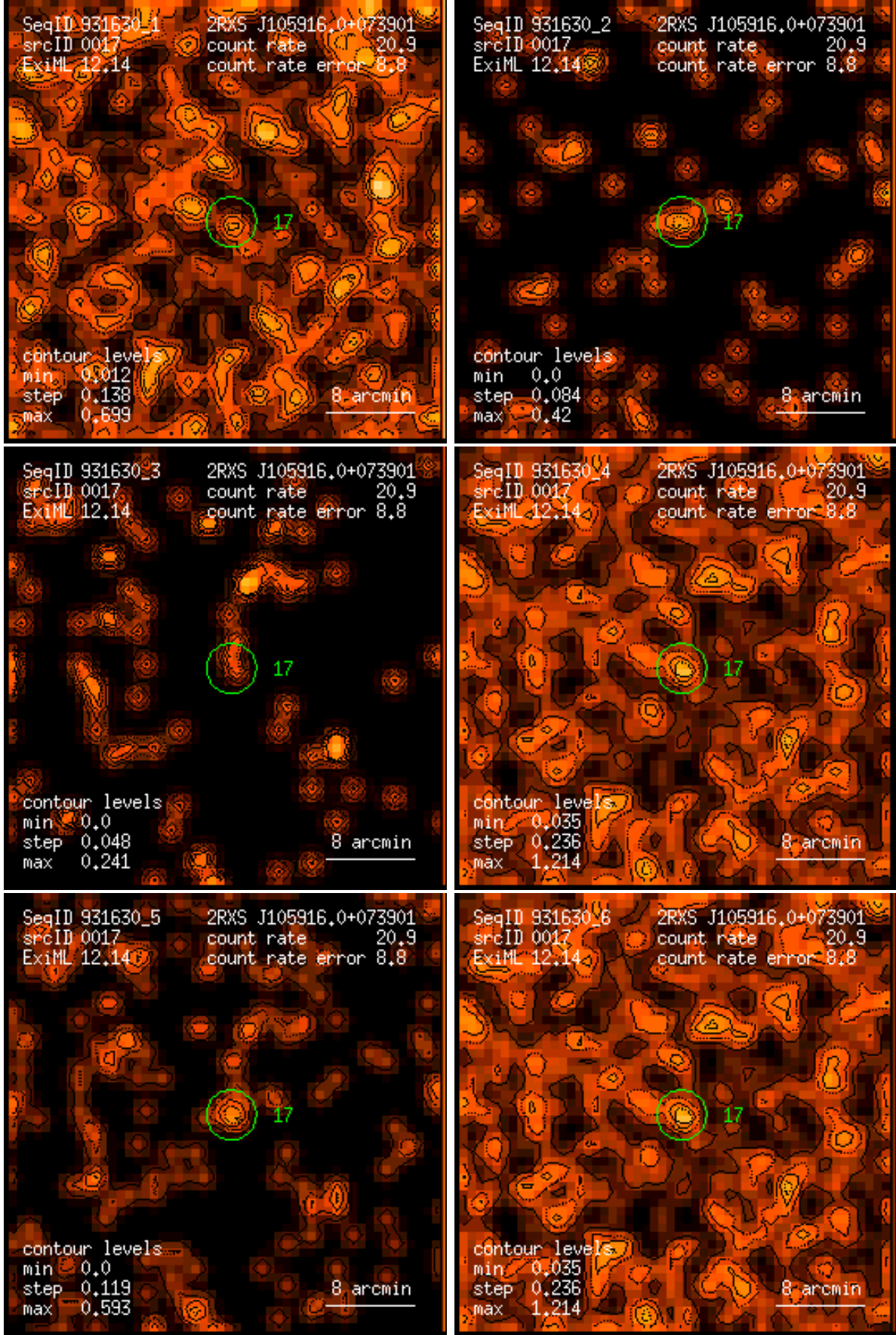
Figure 17: RASS 931630: detection 0017: band rate images, Gaussian filter: (1) PSPC channels 11 – 41, (2) 52 – 90, (3) 91 – 201, (4) 11 – 235, (5) 52 – 201, (6) 11 – 201. Broad band rates in counts/ks. Band rate contour levels in counts/ks/arcmin 2 .
