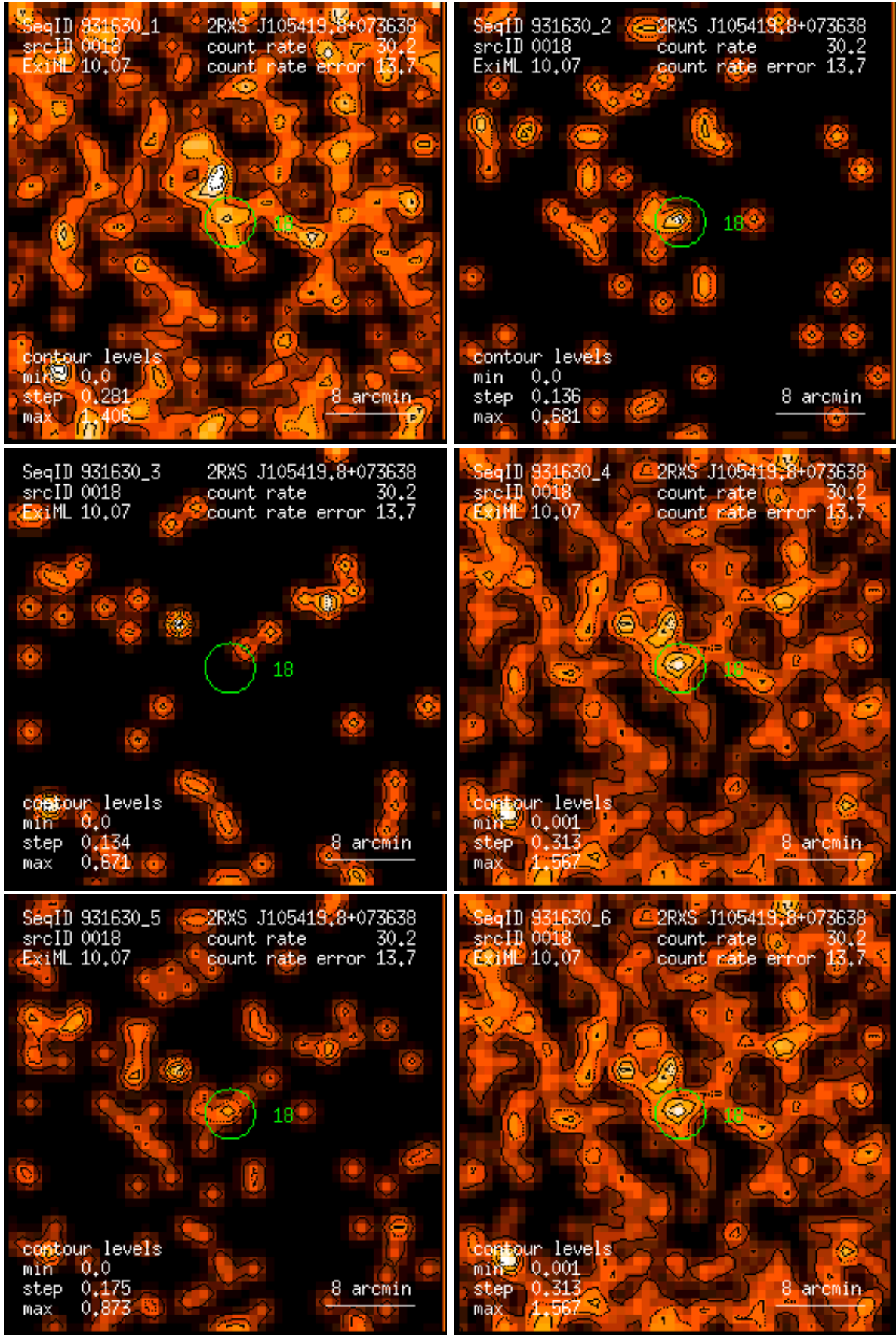
Figure 18: RASS 931630: detection 0018: band rate images, Gaussian filter: (1) PSPC channels 11 – 41, (2) 52 – 90, (3) 91 – 201, (4) 11 – 235, (5) 52 – 201, (6) 11 – 201. Broad band rates in counts/ks. Band rate contour levels in counts/ks/arcmin 2 .
