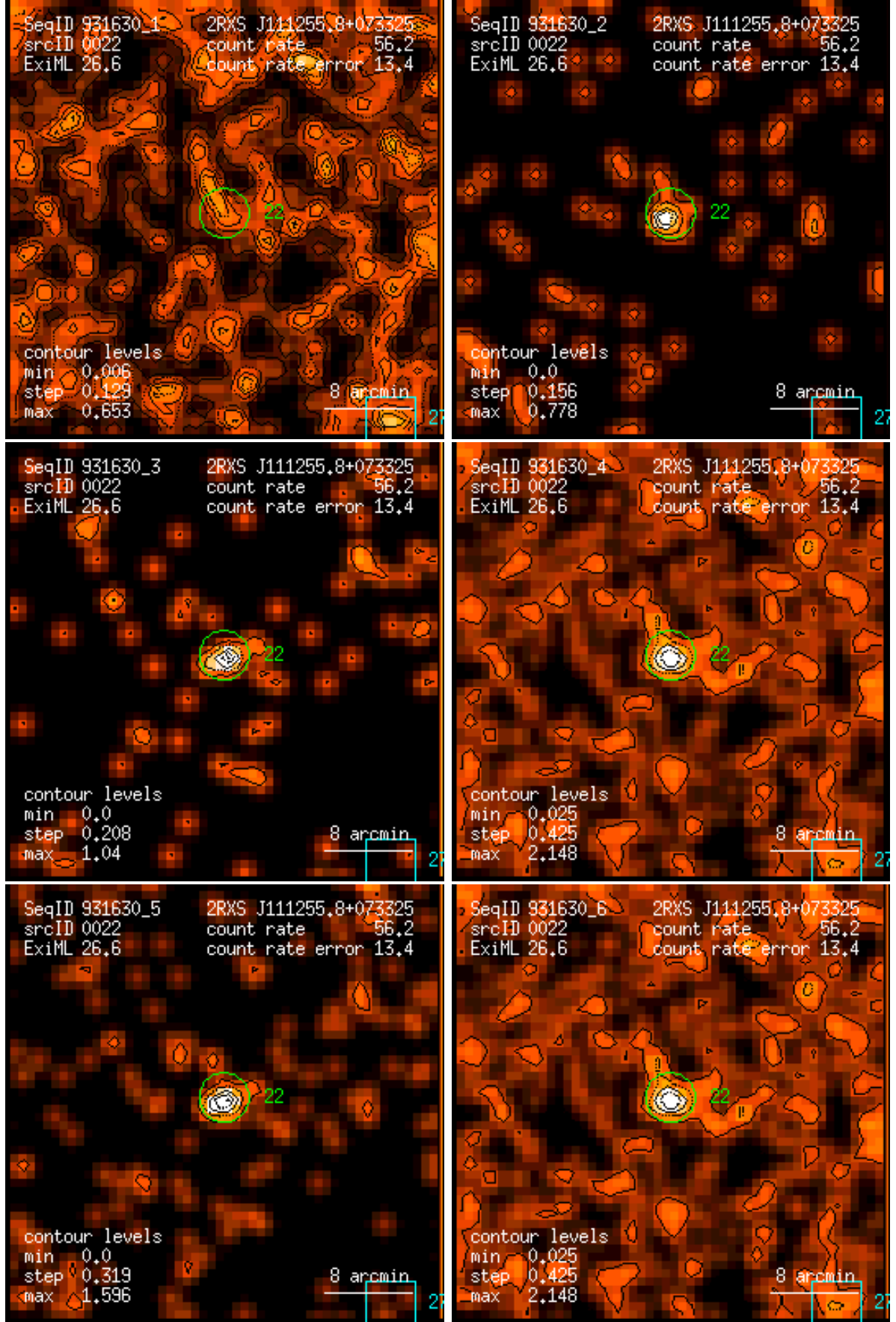
Figure 22: RASS 931630: detection 0022: band rate images, Gaussian filter: (1) PSPC channels 11 – 41, (2) 52 – 90, (3) 91 – 201, (4) 11 – 235, (5) 52 – 201, (6) 11 – 201. Broad band rates in counts/ks. Band rate contour levels in counts/ks/arcmin 2 .
