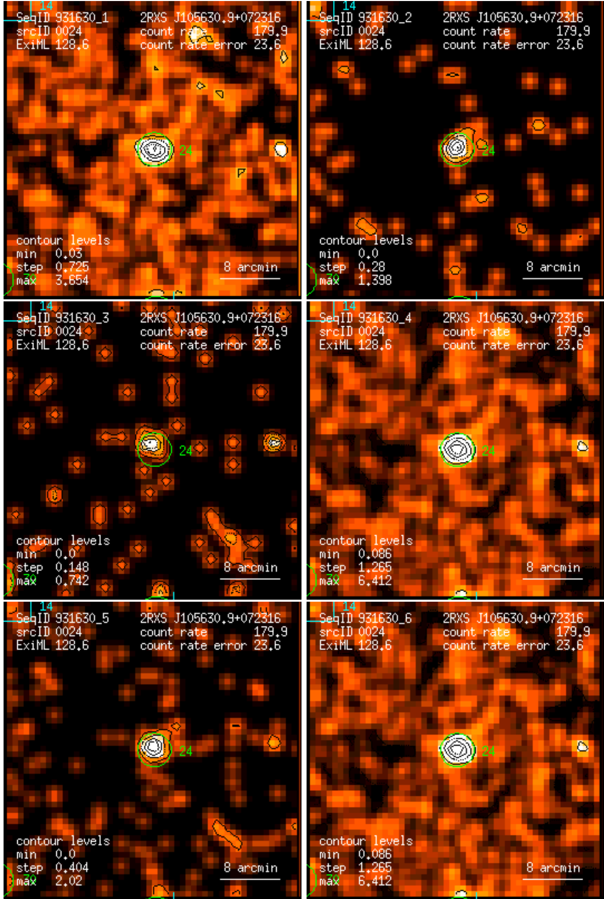
Figure 24: RASS 931630: detection 0024: band rate images, Gaussian filter: (1) PSPC channels 11 – 41, (2) 52 – 90, (3) 91 – 201, (4) 11 – 235, (5) 52 – 201, (6) 11 – 201. Broad band rates in counts/ks. Band rate contour levels in counts/ks/arcmin 2 .
