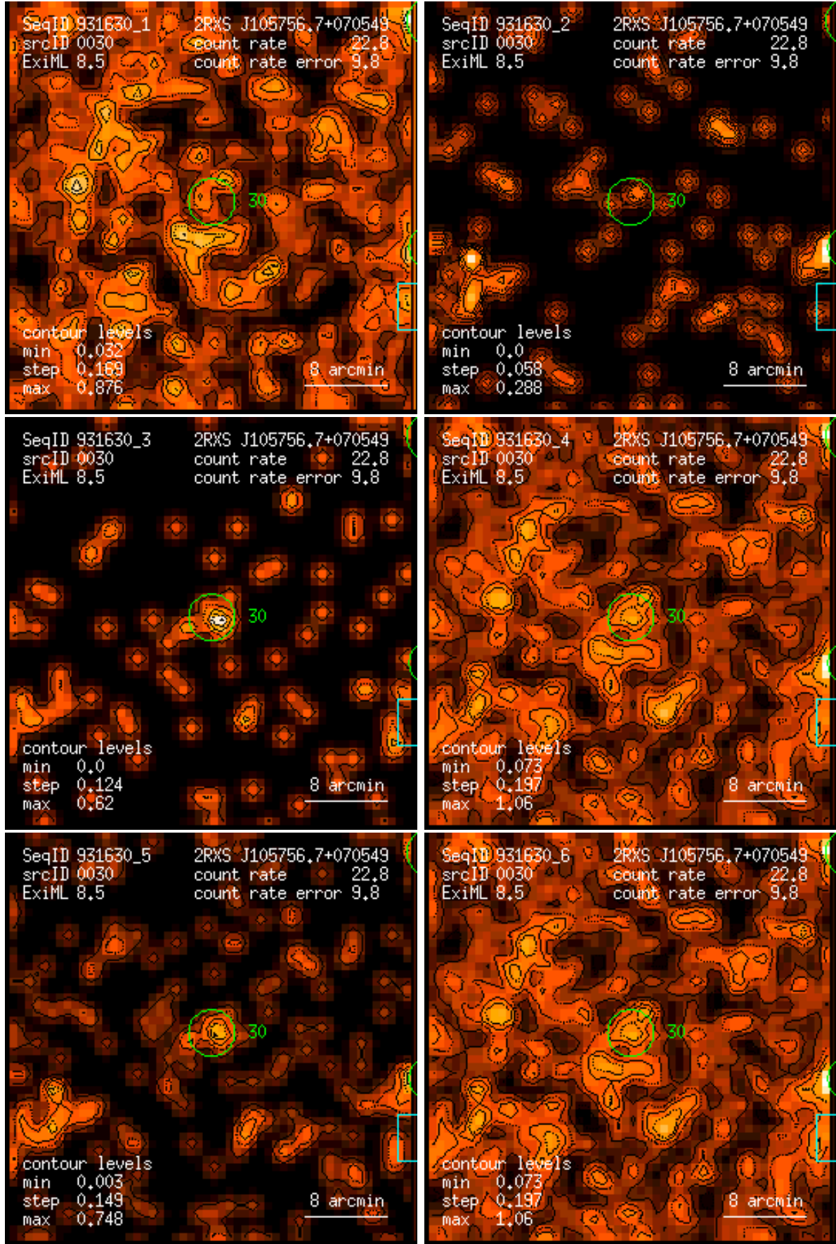
Figure 30: RASS 931630: detection 0030: band rate images, Gaussian filter: (1) PSPC channels 11 – 41, (2) 52 – 90, (3) 91 – 201, (4) 11 – 235, (5) 52 – 201, (6) 11 – 201. Broad band rates in counts/ks. Band rate contour levels in counts/ks/arcmin 2 .
