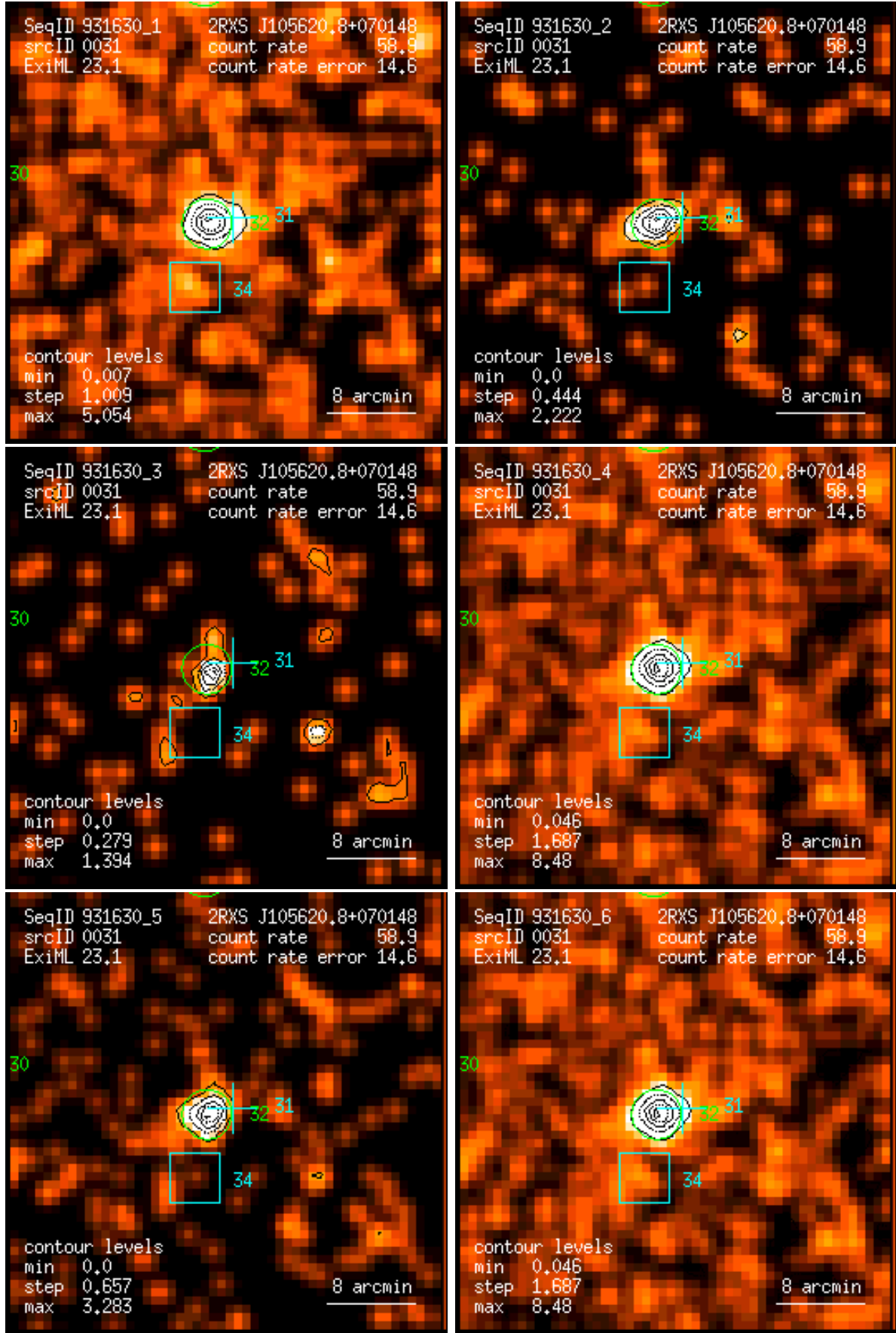
Figure 31: RASS 931630: detection 0031: band rate images, Gaussian filter: (1) PSPC channels 11 – 41, (2) 52 – 90, (3) 91 – 201, (4) 11 – 235, (5) 52 – 201, (6) 11 – 201. Broad band rates in counts/ks. Band rate contour levels in counts/ks/arcmin 2 .
