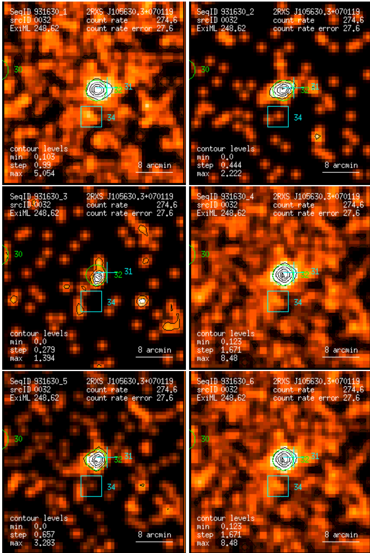
Figure 32: RASS 931630: detection 0032: band rate images, Gaussian filter: (1) PSPC channels 11 – 41, (2) 52 – 90, (3) 91 – 201, (4) 11 – 235, (5) 52 – 201, (6) 11 – 201. Broad band rates in counts/ks. Band rate contour levels in counts/ks/arcmin 2 .
