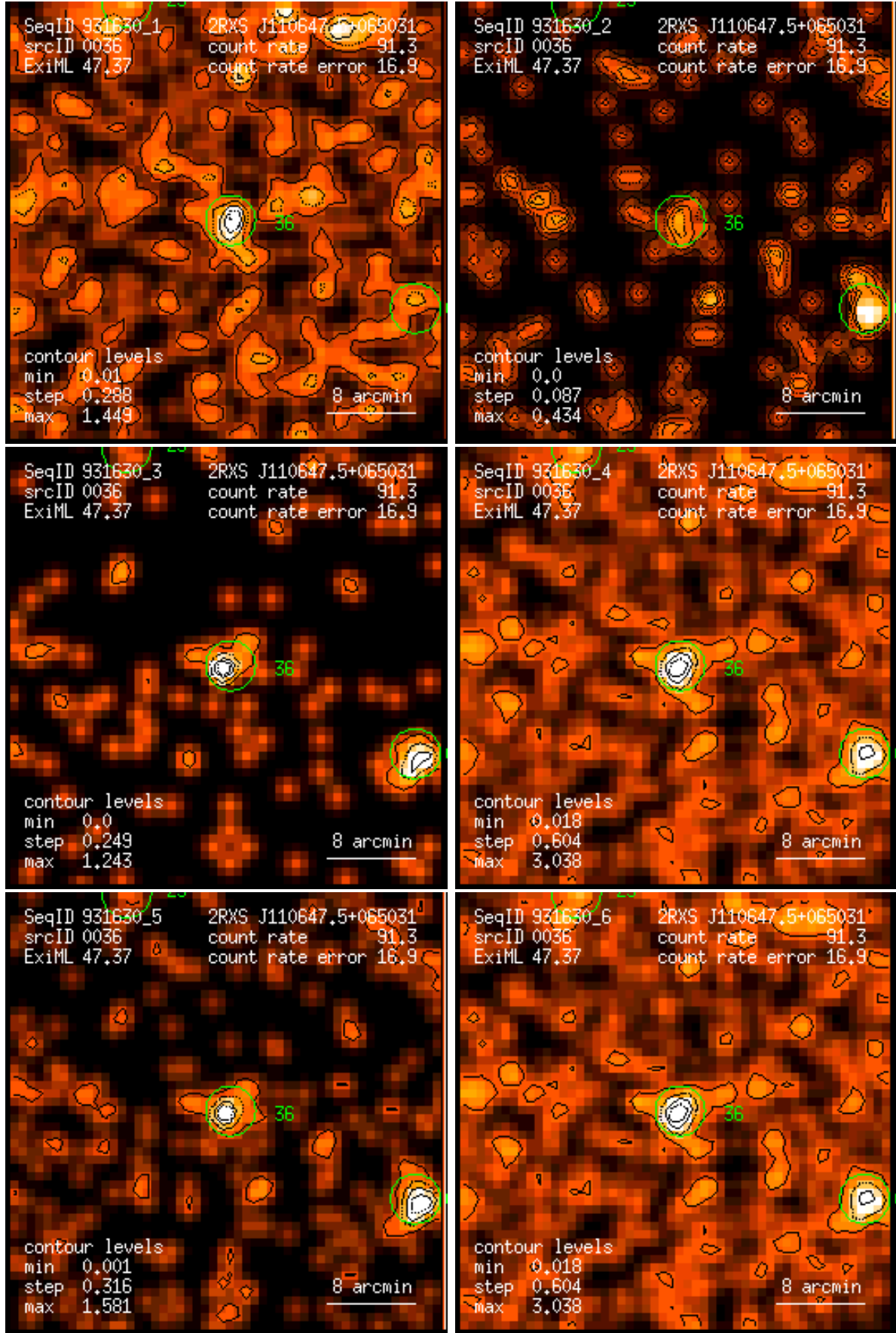
Figure 36: RASS 931630: detection 0036: band rate images, Gaussian filter: (1) PSPC channels 11 – 41, (2) 52 – 90, (3) 91 – 201, (4) 11 – 235, (5) 52 – 201, (6) 11 – 201. Broad band rates in counts/ks. Band rate contour levels in counts/ks/arcmin 2 .
