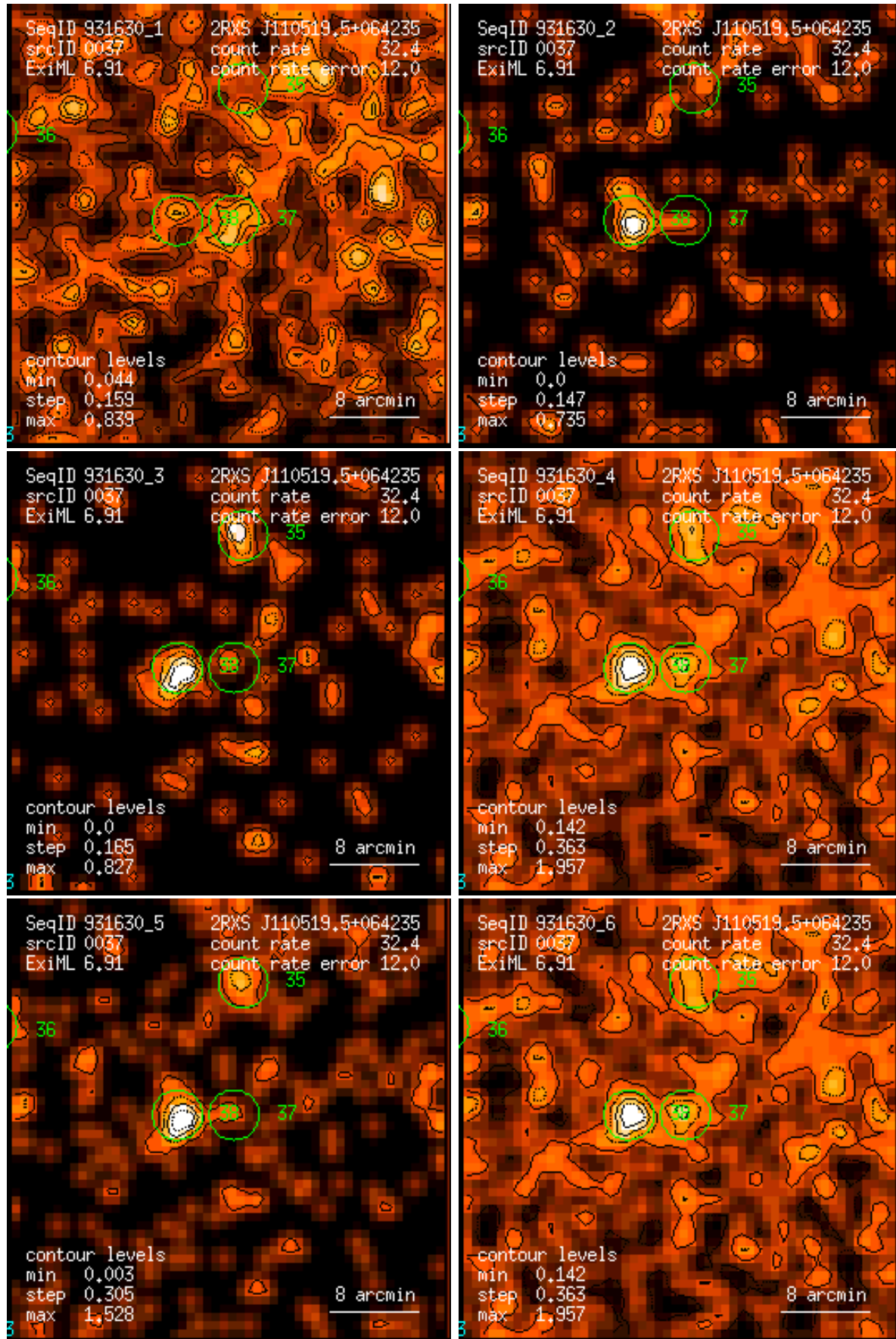
Figure 37: RASS 931630: detection 0037: band rate images, Gaussian filter: (1) PSPC channels 11 – 41, (2) 52 – 90, (3) 91 – 201, (4) 11 – 235, (5) 52 – 201, (6) 11 – 201. Broad band rates in counts/ks. Band rate contour levels in counts/ks/arcmin 2 .
