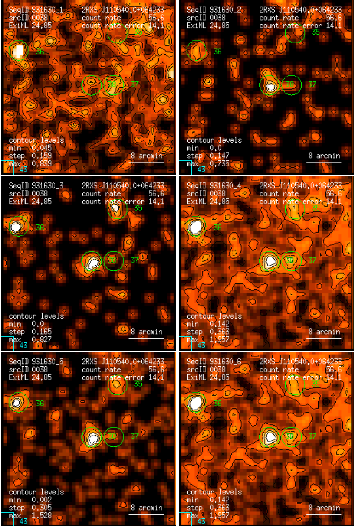
Figure 38: RASS 931630: detection 0038: band rate images, Gaussian filter: (1) PSPC channels 11 – 41, (2) 52 – 90, (3) 91 – 201, (4) 11 – 235, (5) 52 – 201, (6) 11 – 201. Broad band rates in counts/ks. Band rate contour levels in counts/ks/arcmin 2 .
