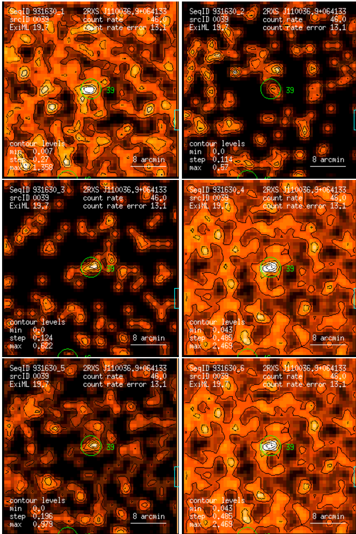
Figure 39: RASS 931630: detection 0039: band rate images, Gaussian filter: (1) PSPC channels 11 – 41, (2) 52 – 90, (3) 91 – 201, (4) 11 – 235, (5) 52 – 201, (6) 11 – 201. Broad band rates in counts/ks. Band rate contour levels in counts/ks/arcmin 2 .
