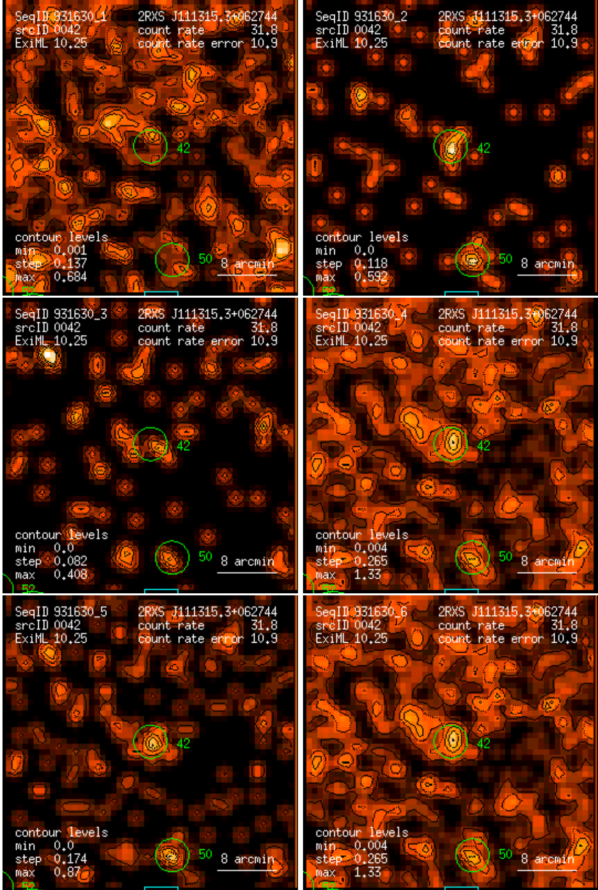
Figure 42: RASS 931630: detection 0042: band rate images, Gaussian filter: (1) PSPC channels 11 – 41, (2) 52 – 90, (3) 91 – 201, (4) 11 – 235, (5) 52 – 201, (6) 11 – 201. Broad band rates in counts/ks. Band rate contour levels in counts/ks/arcmin 2 .
