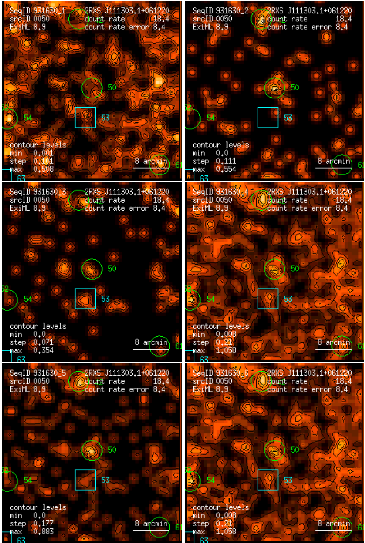
Figure 50: RASS 931630: detection 0050: band rate images, Gaussian filter: (1) PSPC channels 11 – 41, (2) 52 – 90, (3) 91 – 201, (4) 11 – 235, (5) 52 – 201, (6) 11 – 201. Broad band rates in counts/ks. Band rate contour levels in counts/ks/arcmin 2 .
