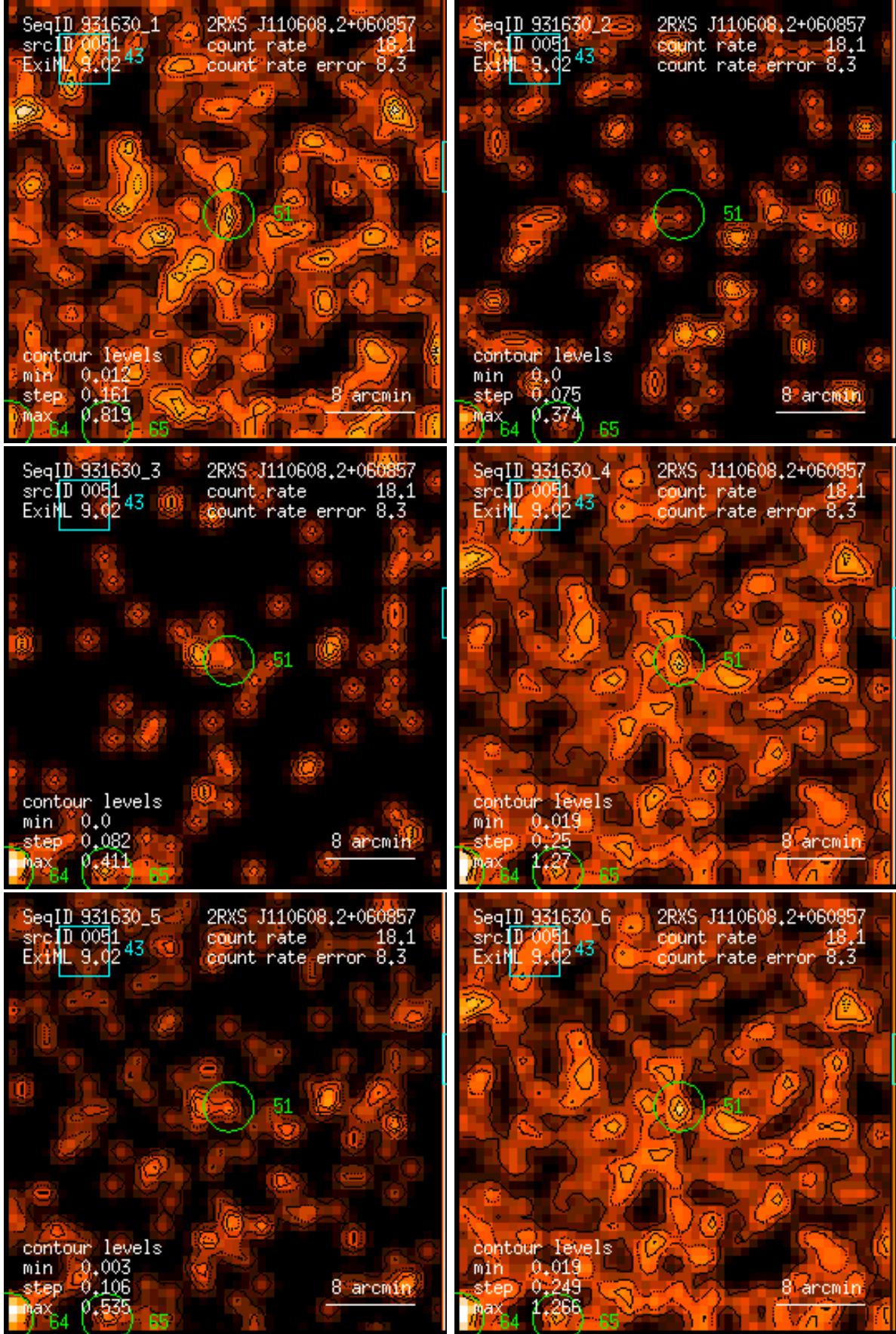
Figure 51: RASS 931630: detection 0051: band rate images, Gaussian filter: (1) PSPC channels 11 – 41, (2) 52 – 90, (3) 91 – 201, (4) 11 – 235, (5) 52 – 201, (6) 11 – 201. Broad band rates in counts/ks. Band rate contour levels in counts/ks/arcmin 2 .
