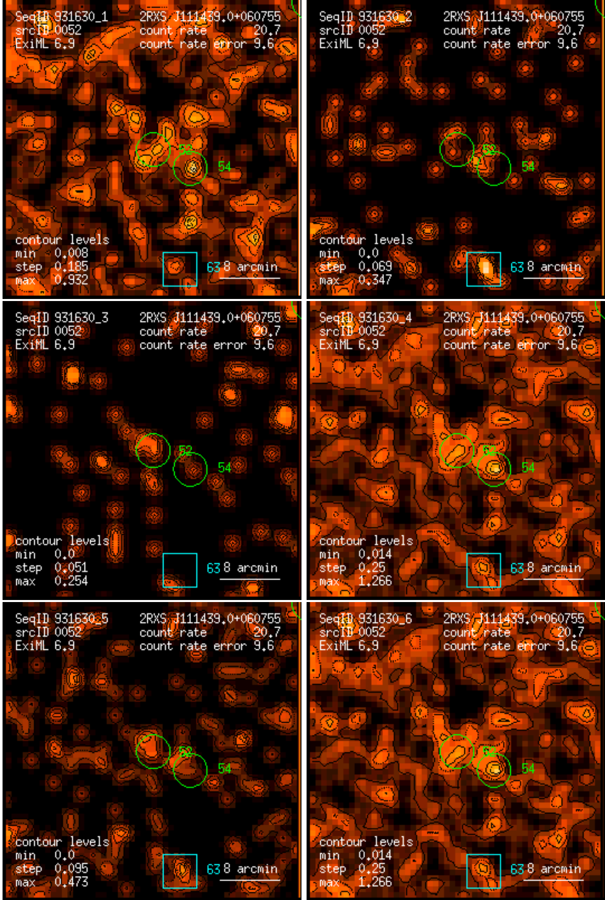
Figure 52: RASS 931630: detection 0052: band rate images, Gaussian filter: (1) PSPC channels 11 – 41, (2) 52 – 90, (3) 91 – 201, (4) 11 – 235, (5) 52 – 201, (6) 11 – 201. Broad band rates in counts/ks. Band rate contour levels in counts/ks/arcmin 2 .
