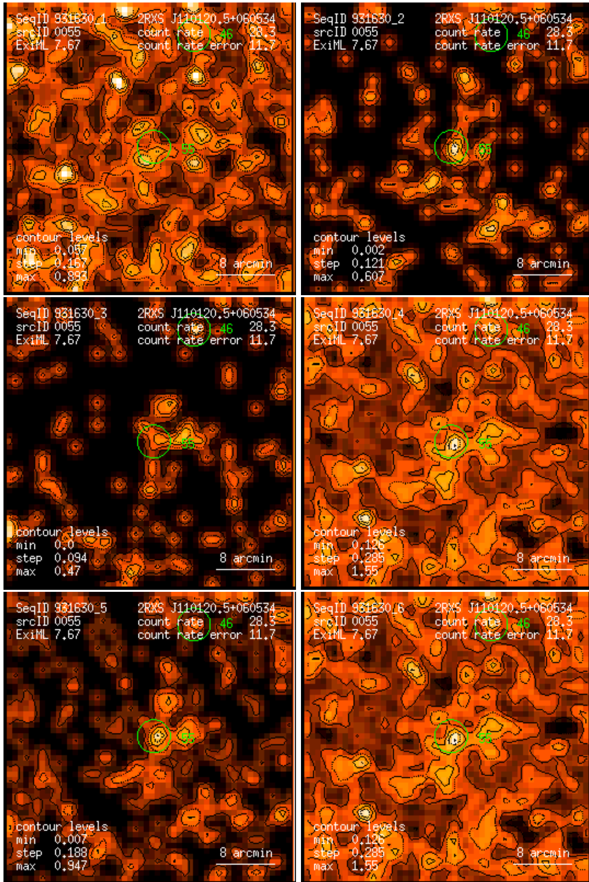
Figure 55: RASS 931630: detection 0055: band rate images, Gaussian filter: (1) PSPC channels 11 – 41, (2) 52 – 90, (3) 91 – 201, (4) 11 – 235, (5) 52 – 201, (6) 11 – 201. Broad band rates in counts/ks. Band rate contour levels in counts/ks/arcmin 2 .
