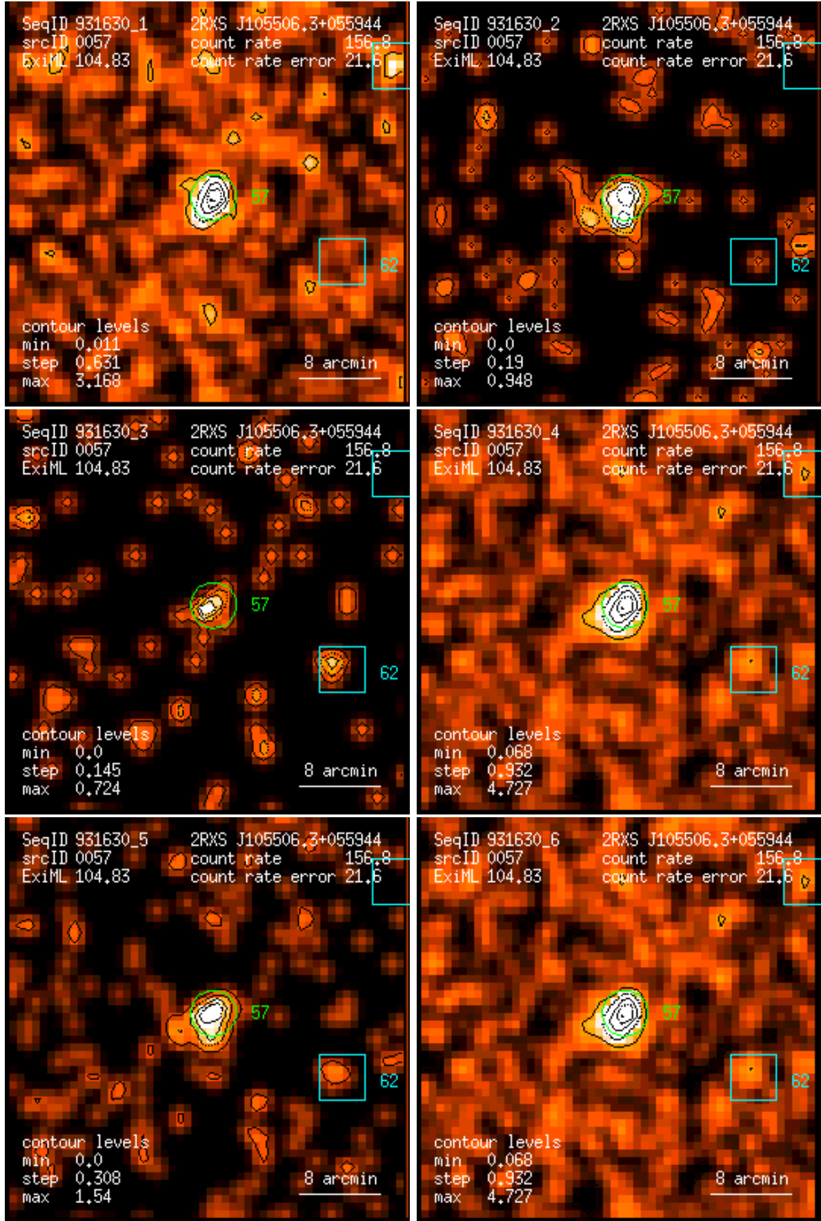
Figure 57: RASS 931630: detection 0057: band rate images, Gaussian filter: (1) PSPC channels 11 – 41, (2) 52 – 90, (3) 91 – 201, (4) 11 – 235, (5) 52 – 201, (6) 11 – 201. Broad band rates in counts/ks. Band rate contour levels in counts/ks/arcmin 2 .
