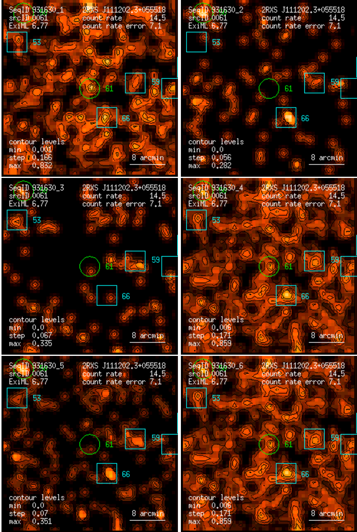
Figure 61: RASS 931630: detection 0061: band rate images, Gaussian filter: (1) PSPC channels 11 – 41, (2) 52 – 90, (3) 91 – 201, (4) 11 – 235, (5) 52 – 201, (6) 11 – 201. Broad band rates in counts/ks. Band rate contour levels in counts/ks/arcmin 2 .
