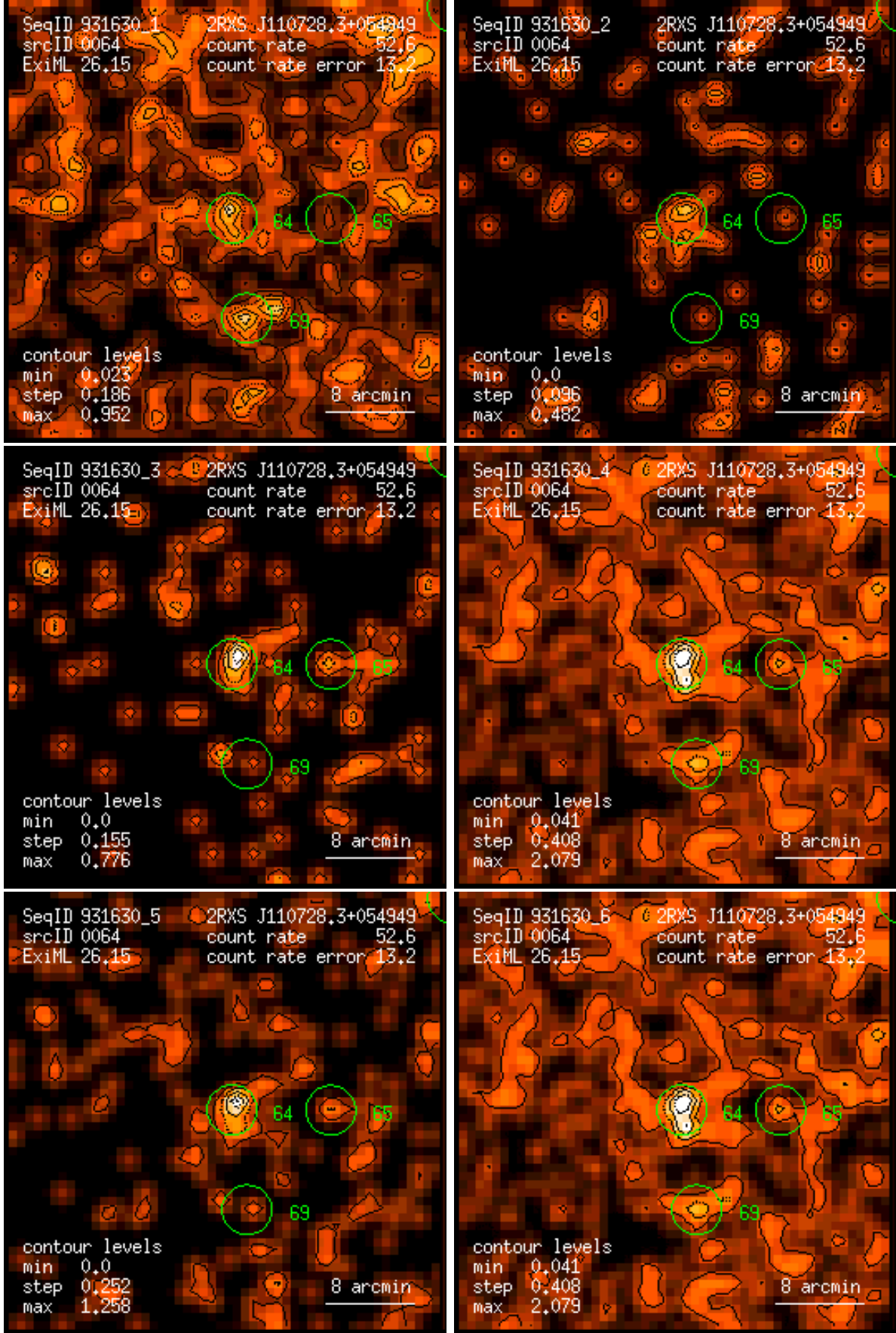
Figure 64: RASS 931630: detection 0064: band rate images, Gaussian filter: (1) PSPC channels 11 – 41, (2) 52 – 90, (3) 91 – 201, (4) 11 – 235, (5) 52 – 201, (6) 11 – 201. Broad band rates in counts/ks. Band rate contour levels in counts/ks/arcmin 2 .
