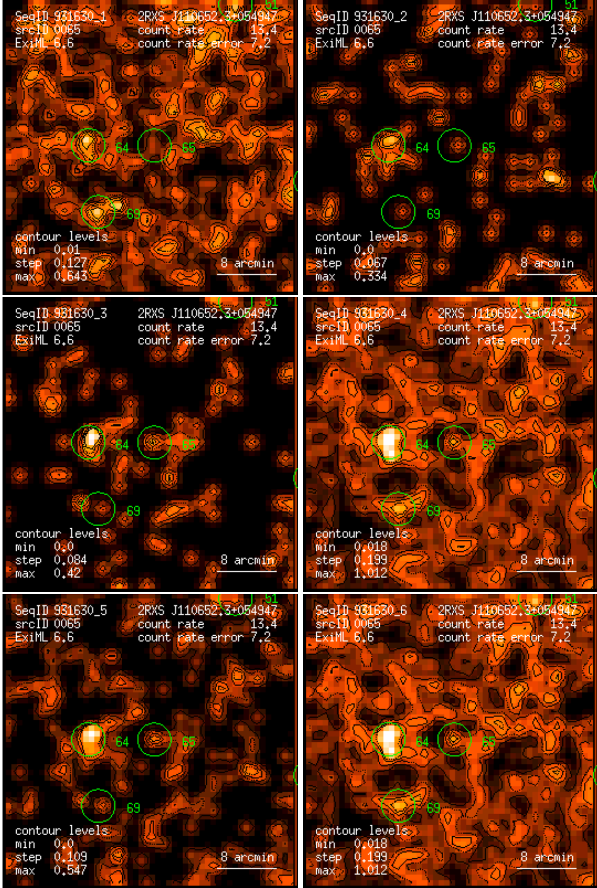
Figure 65: RASS 931630: detection 0065: band rate images, Gaussian filter: (1) PSPC channels 11 – 41, (2) 52 – 90, (3) 91 – 201, (4) 11 – 235, (5) 52 – 201, (6) 11 – 201. Broad band rates in counts/ks. Band rate contour levels in counts/ks/arcmin 2 .
