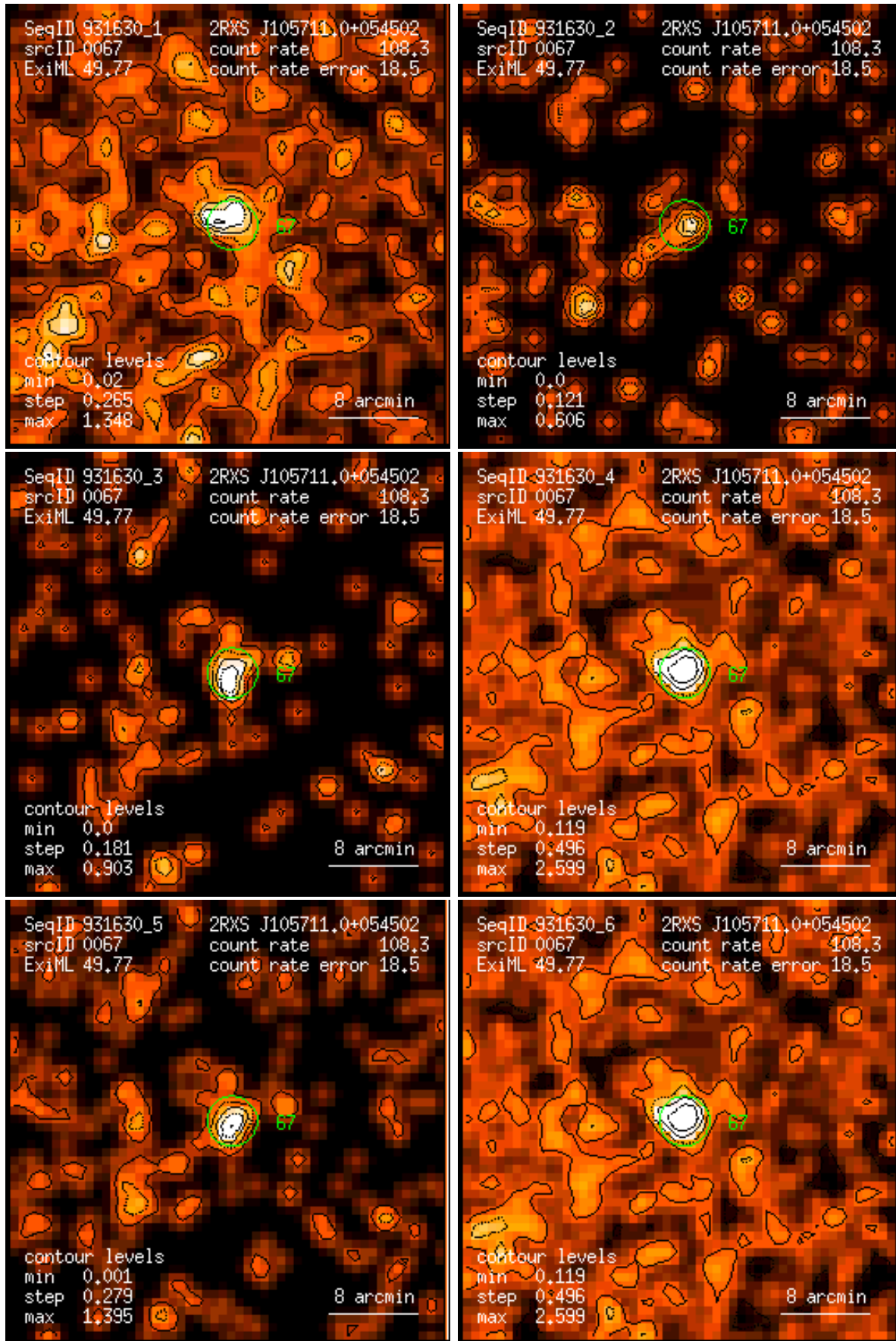
Figure 67: RASS 931630: detection 0067: band rate images, Gaussian filter: (1) PSPC channels 11 – 41, (2) 52 – 90, (3) 91 – 201, (4) 11 – 235, (5) 52 – 201, (6) 11 – 201. Broad band rates in counts/ks. Band rate contour levels in counts/ks/arcmin 2 .
