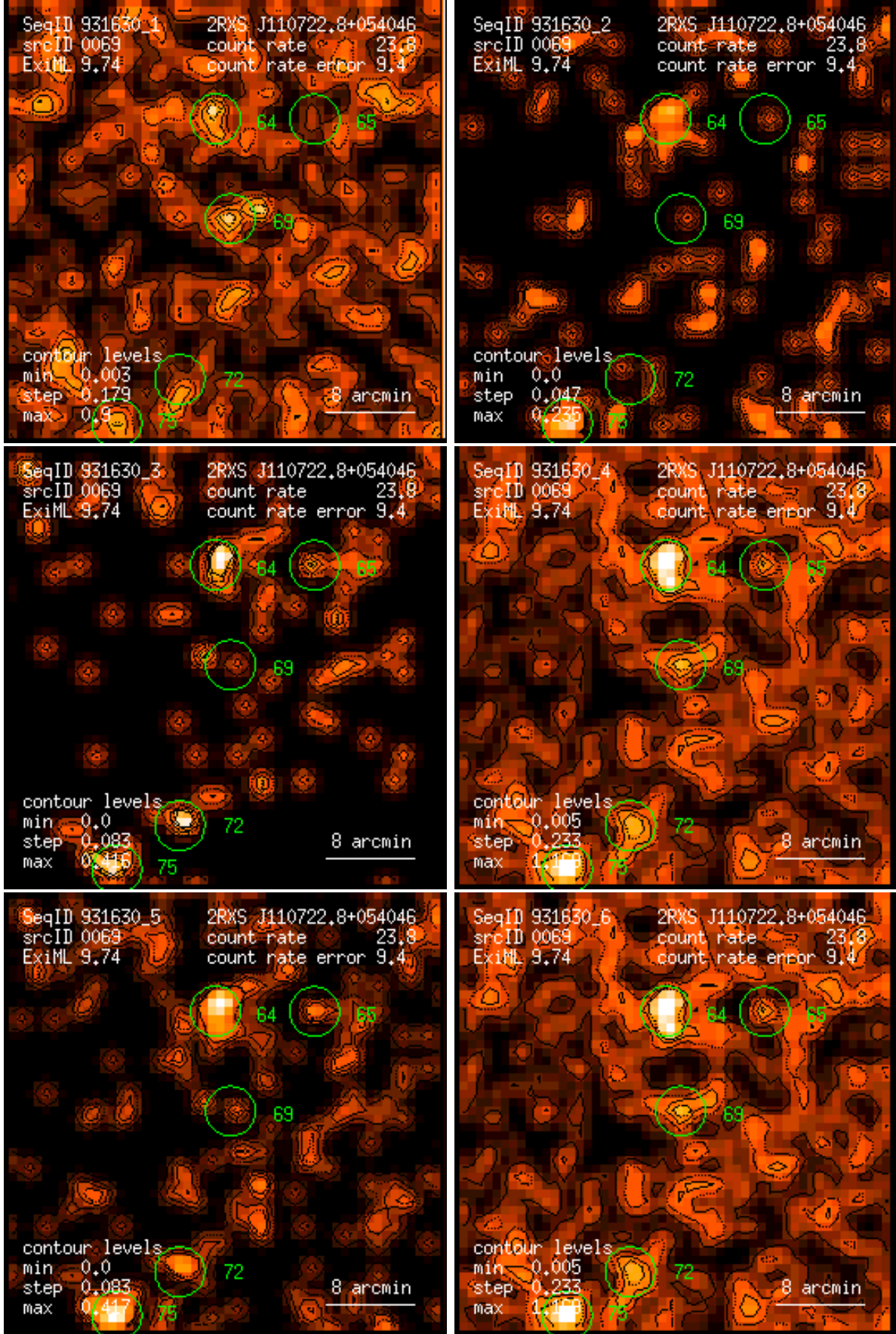
Figure 69: RASS 931630: detection 0069: band rate images, Gaussian filter: (1) PSPC channels 11 – 41, (2) 52 – 90, (3) 91 – 201, (4) 11 – 235, (5) 52 – 201, (6) 11 – 201. Broad band rates in counts/ks. Band rate contour levels in counts/ks/arcmin 2 .
