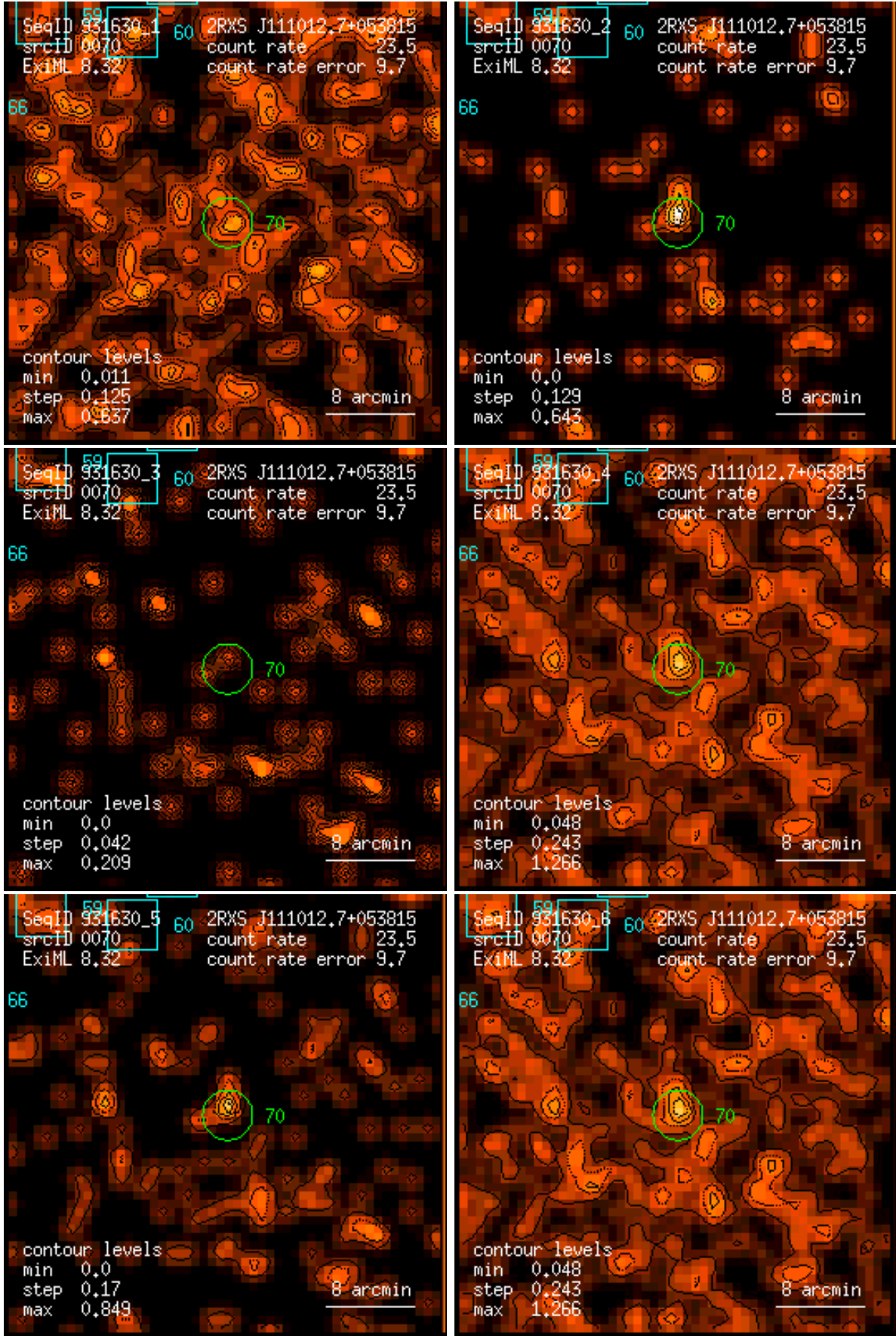
Figure 70: RASS 931630: detection 0070: band rate images, Gaussian filter: (1) PSPC channels 11 – 41, (2) 52 – 90, (3) 91 – 201, (4) 11 – 235, (5) 52 – 201, (6) 11 – 201. Broad band rates in counts/ks. Band rate contour levels in counts/ks/arcmin 2 .
