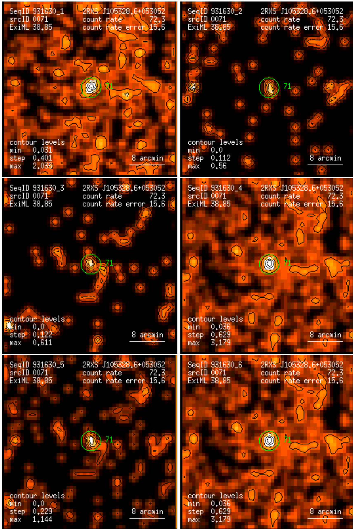
Figure 71: RASS 931630: detection 0071: band rate images, Gaussian filter: (1) PSPC channels 11 – 41, (2) 52 – 90, (3) 91 – 201, (4) 11 – 235, (5) 52 – 201, (6) 11 – 201. Broad band rates in counts/ks. Band rate contour levels in counts/ks/arcmin 2 .
