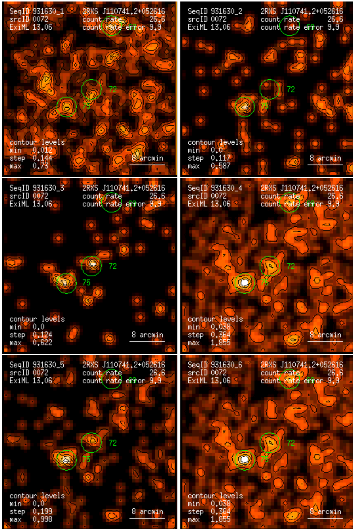
Figure 72: RASS 931630: detection 0072: band rate images, Gaussian filter: (1) PSPC channels 11 – 41, (2) 52 – 90, (3) 91 – 201, (4) 11 – 235, (5) 52 – 201, (6) 11 – 201. Broad band rates in counts/ks. Band rate contour levels in counts/ks/arcmin 2 .
