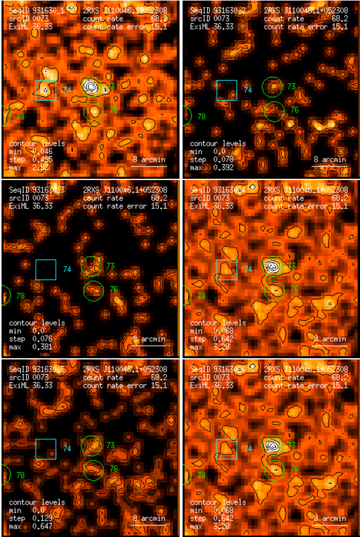
Figure 73: RASS 931630: detection 0073: band rate images, Gaussian filter: (1) PSPC channels 11 – 41, (2) 52 – 90, (3) 91 – 201, (4) 11 – 235, (5) 52 – 201, (6) 11 – 201. Broad band rates in counts/ks. Band rate contour levels in counts/ks/arcmin 2 .
