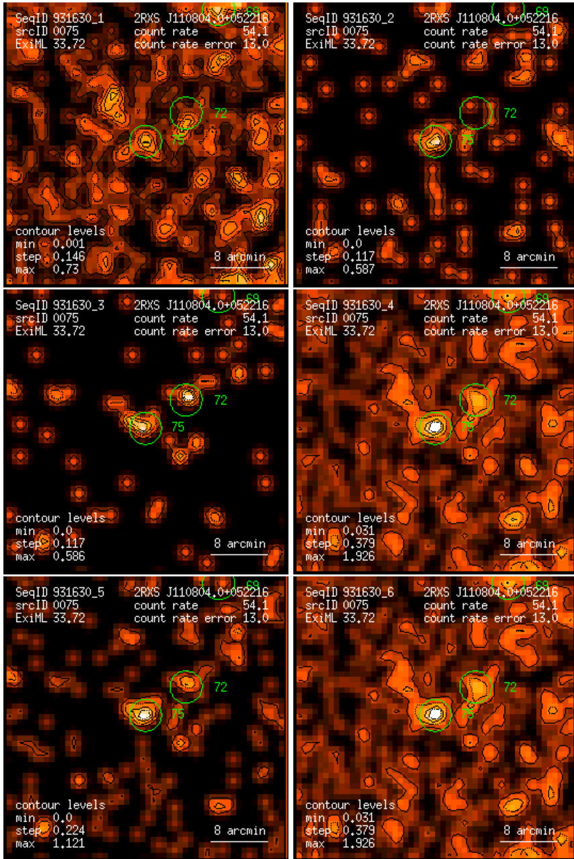
Figure 75: RASS 931630: detection 0075: band rate images, Gaussian filter: (1) PSPC channels 11 – 41, (2) 52 – 90, (3) 91 – 201, (4) 11 – 235, (5) 52 – 201, (6) 11 – 201. Broad band rates in counts/ks. Band rate contour levels in counts/ks/arcmin 2 .
