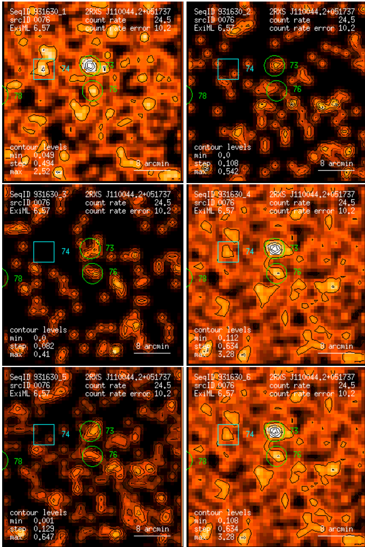
Figure 76: RASS 931630: detection 0076: band rate images, Gaussian filter: (1) PSPC channels 11 – 41, (2) 52 – 90, (3) 91 – 201, (4) 11 – 235, (5) 52 – 201, (6) 11 – 201. Broad band rates in counts/ks. Band rate contour levels in counts/ks/arcmin 2 .
