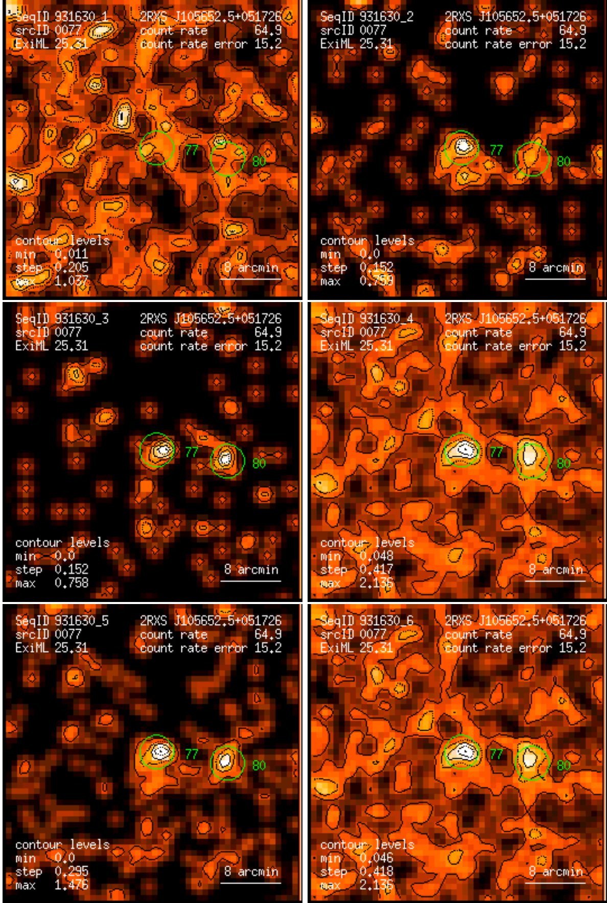
Figure 77: RASS 931630: detection 0077: band rate images, Gaussian filter: (1) PSPC channels 11 – 41, (2) 52 – 90, (3) 91 – 201, (4) 11 – 235, (5) 52 – 201, (6) 11 – 201. Broad band rates in counts/ks. Band rate contour levels in counts/ks/arcmin 2 .
