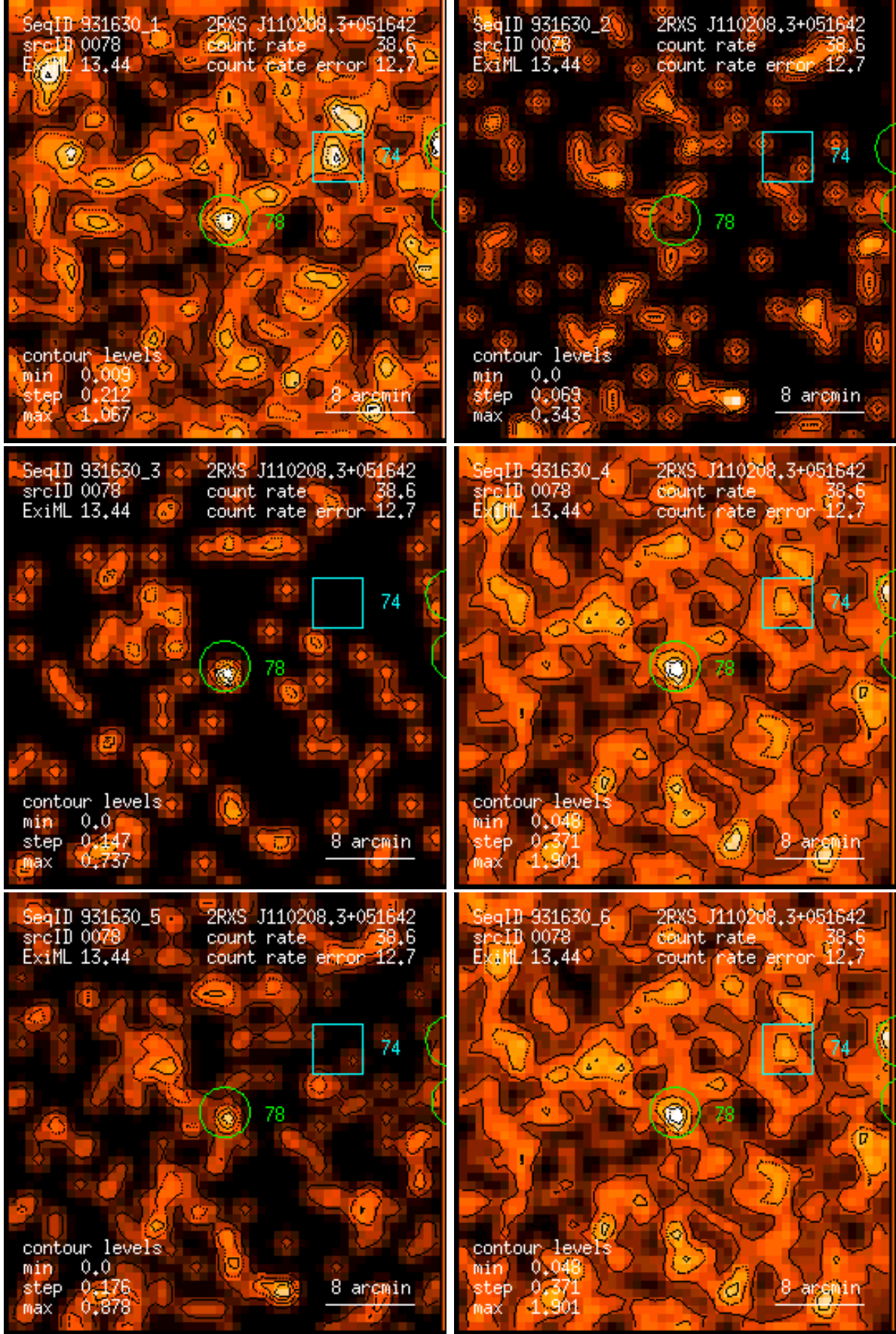
Figure 78: RASS 931630: detection 0078: band rate images, Gaussian filter: (1) PSPC channels 11 – 41, (2) 52 – 90, (3) 91 – 201, (4) 11 – 235, (5) 52 – 201, (6) 11 – 201. Broad band rates in counts/ks. Band rate contour levels in counts/ks/arcmin 2 .
