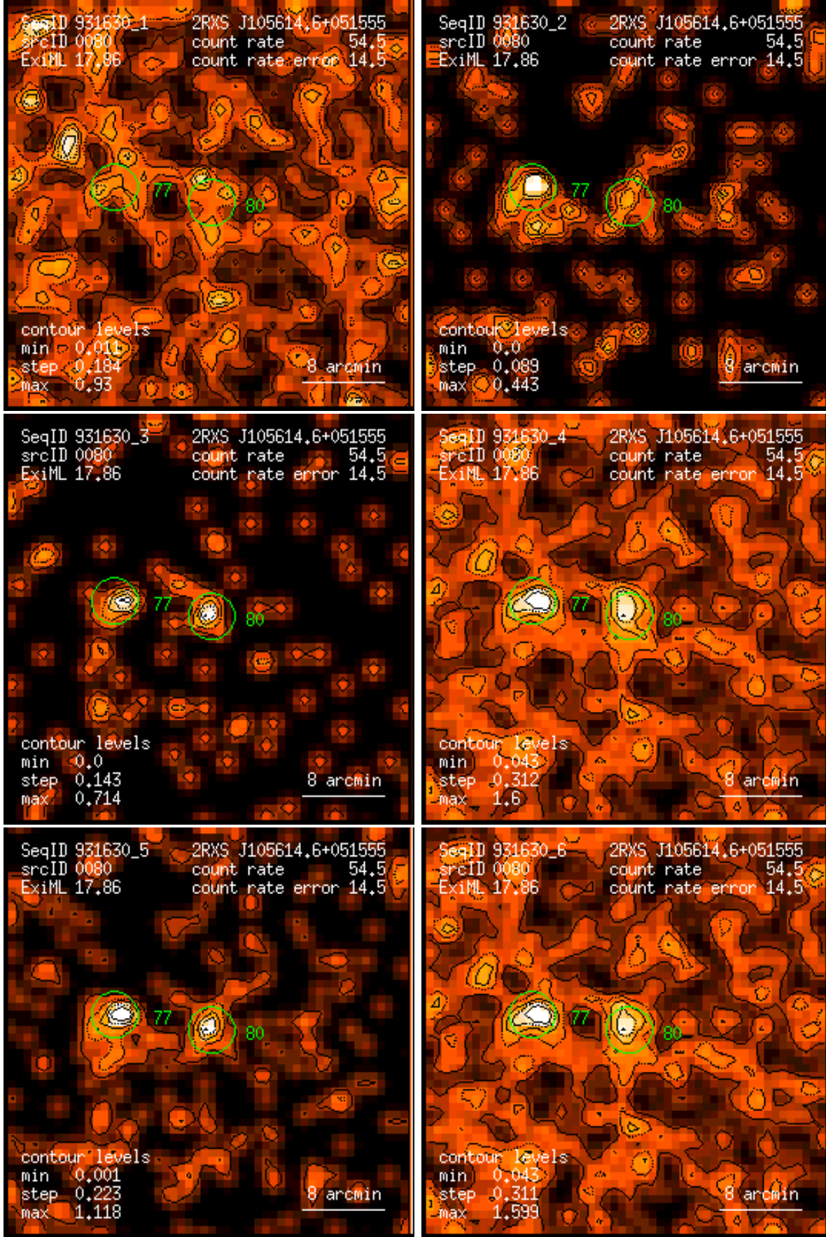
Figure 80: RASS 931630: detection 0080: band rate images, Gaussian filter: (1) PSPC channels 11 – 41, (2) 52 – 90, (3) 91 – 201, (4) 11 – 235, (5) 52 – 201, (6) 11 – 201. Broad band rates in counts/ks. Band rate contour levels in counts/ks/arcmin 2 .
