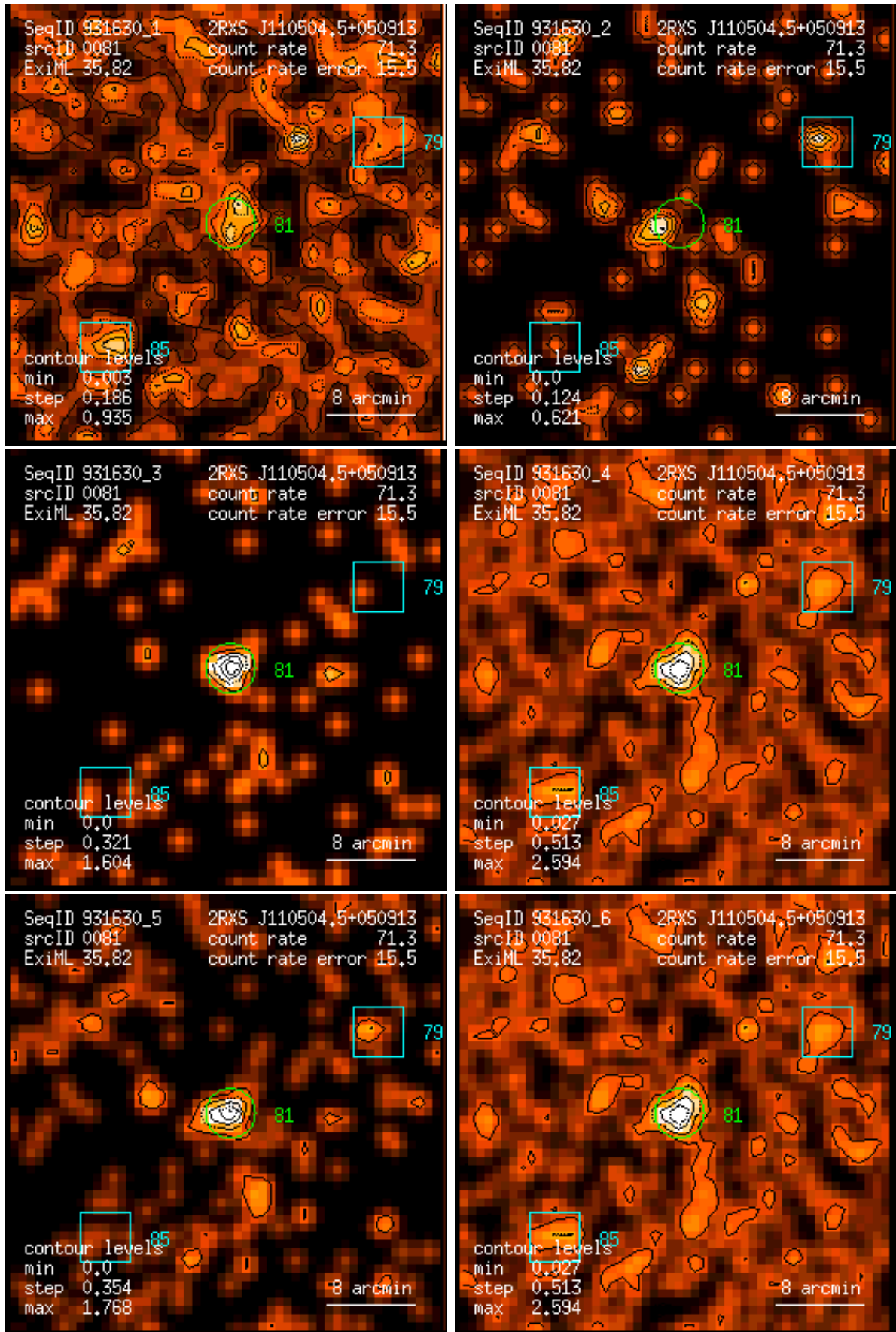
Figure 81: RASS 931630: detection 0081: band rate images, Gaussian filter: (1) PSPC channels 11 – 41, (2) 52 – 90, (3) 91 – 201, (4) 11 – 235, (5) 52 – 201, (6) 11 – 201. Broad band rates in counts/ks. Band rate contour levels in counts/ks/arcmin 2 .
