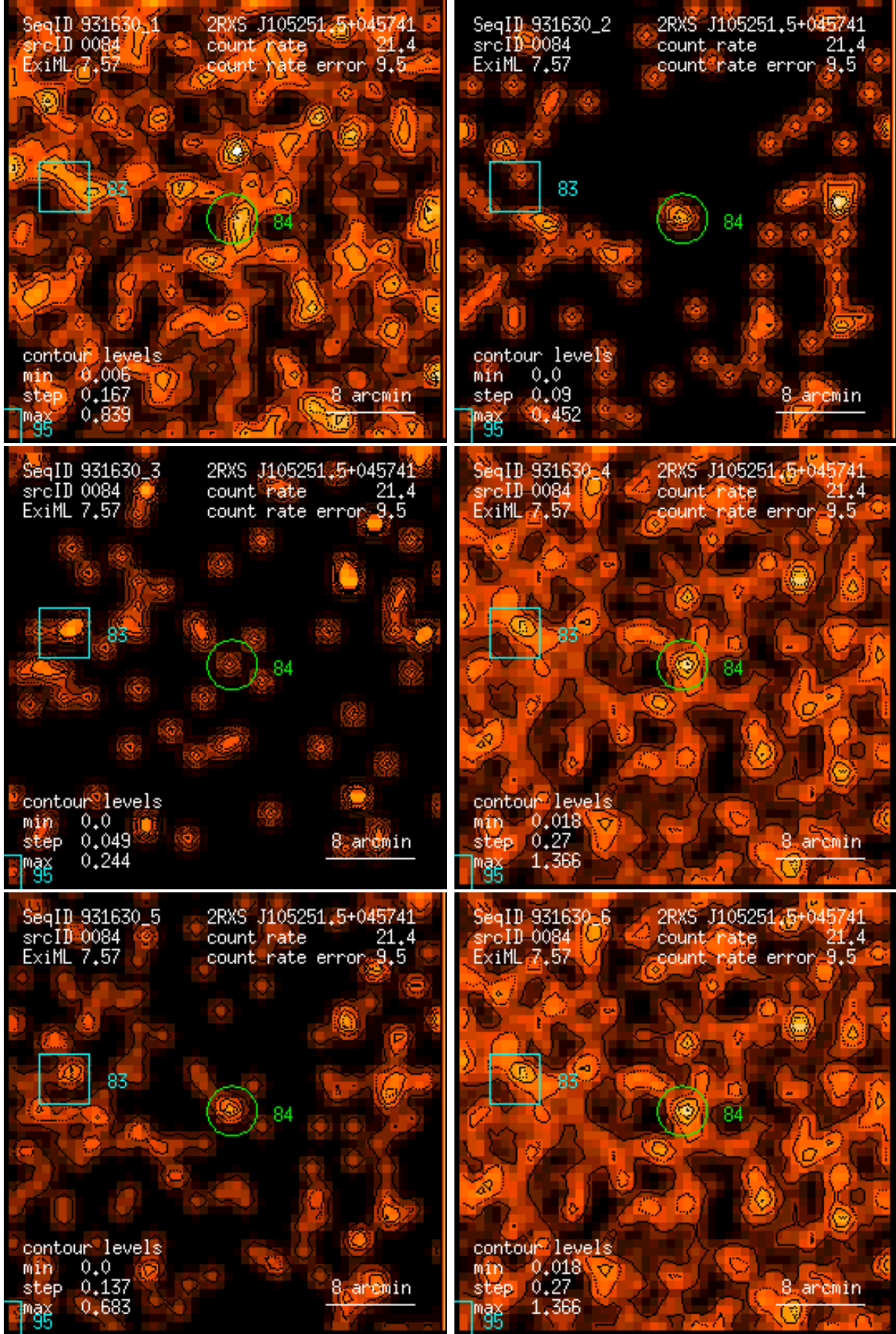
Figure 84: RASS 931630: detection 0084: band rate images, Gaussian filter: (1) PSPC channels 11 – 41, (2) 52 – 90, (3) 91 – 201, (4) 11 – 235, (5) 52 – 201, (6) 11 – 201. Broad band rates in counts/ks. Band rate contour levels in counts/ks/arcmin 2 .
