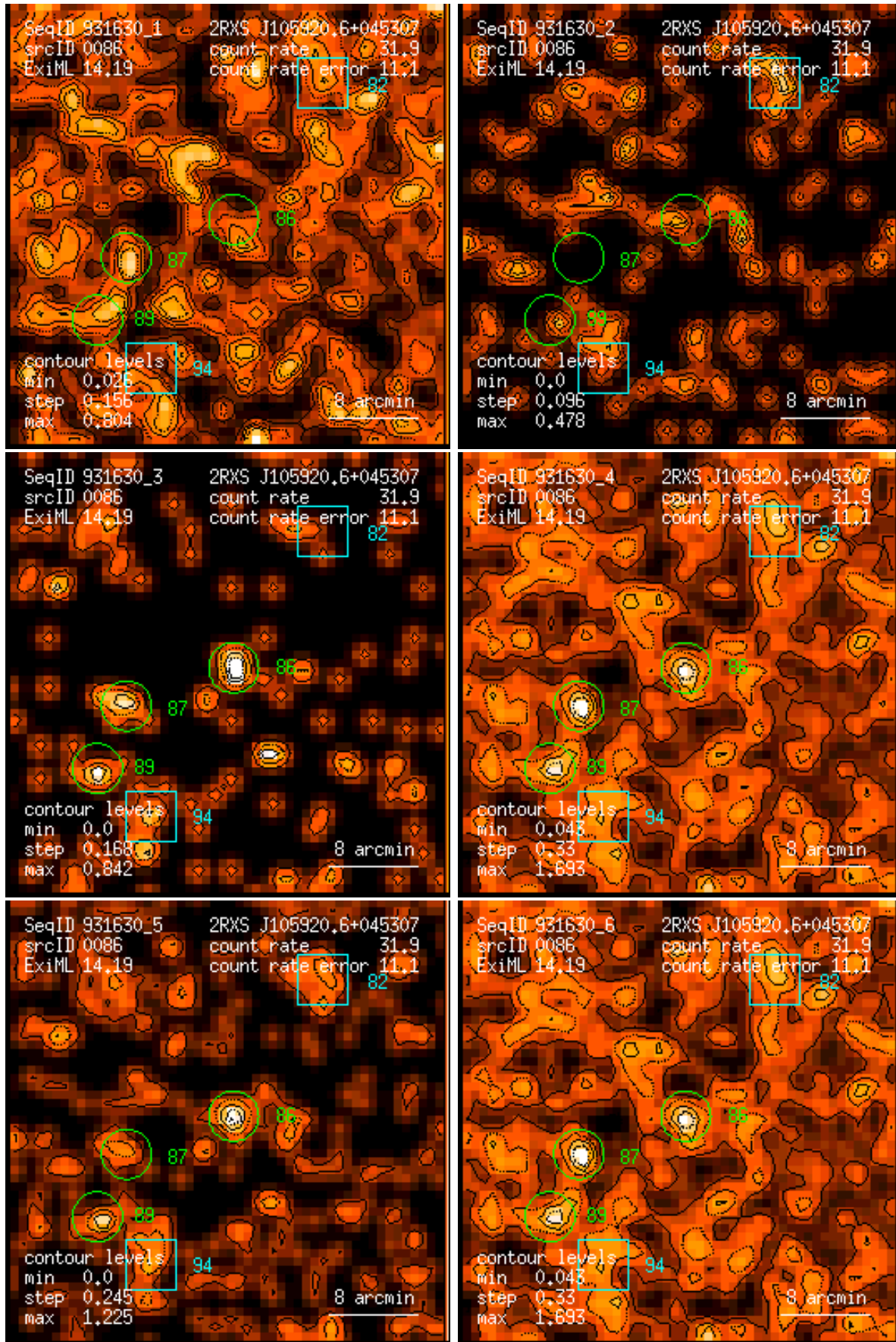
Figure 86: RASS 931630: detection 0086: band rate images, Gaussian filter: (1) PSPC channels 11 – 41, (2) 52 – 90, (3) 91 – 201, (4) 11 – 235, (5) 52 – 201, (6) 11 – 201. Broad band rates in counts/ks. Band rate contour levels in counts/ks/arcmin 2 .
