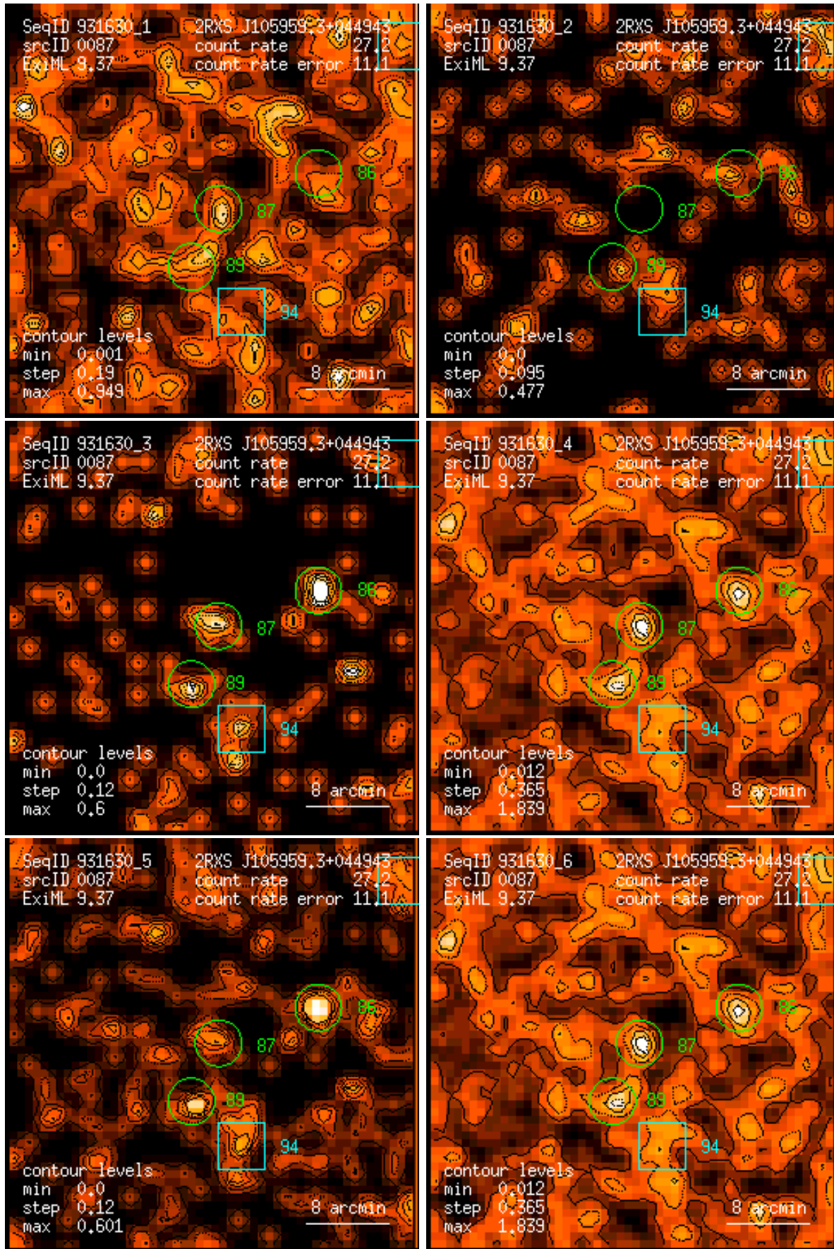
Figure 87: RASS 931630: detection 0087: band rate images, Gaussian filter: (1) PSPC channels 11 – 41, (2) 52 – 90, (3) 91 – 201, (4) 11 – 235, (5) 52 – 201, (6) 11 – 201. Broad band rates in counts/ks. Band rate contour levels in counts/ks/arcmin 2 .
