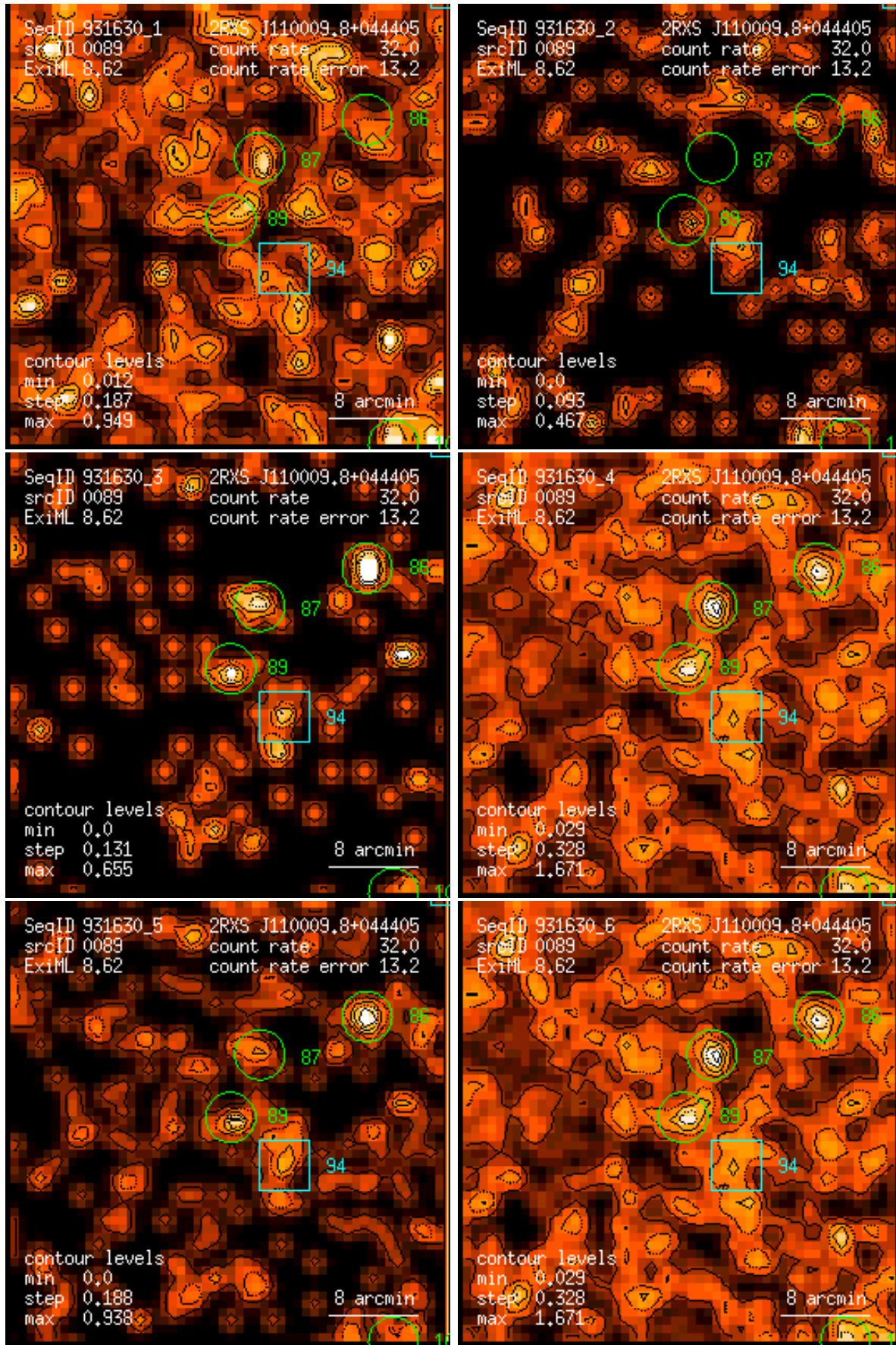
Figure 89: RASS 931630: detection 0089: band rate images, Gaussian filter: (1) PSPC channels 11 – 41, (2) 52 – 90, (3) 91 – 201, (4) 11 – 235, (5) 52 – 201, (6) 11 – 201. Broad band rates in counts/ks. Band rate contour levels in counts/ks/arcmin 2 .
