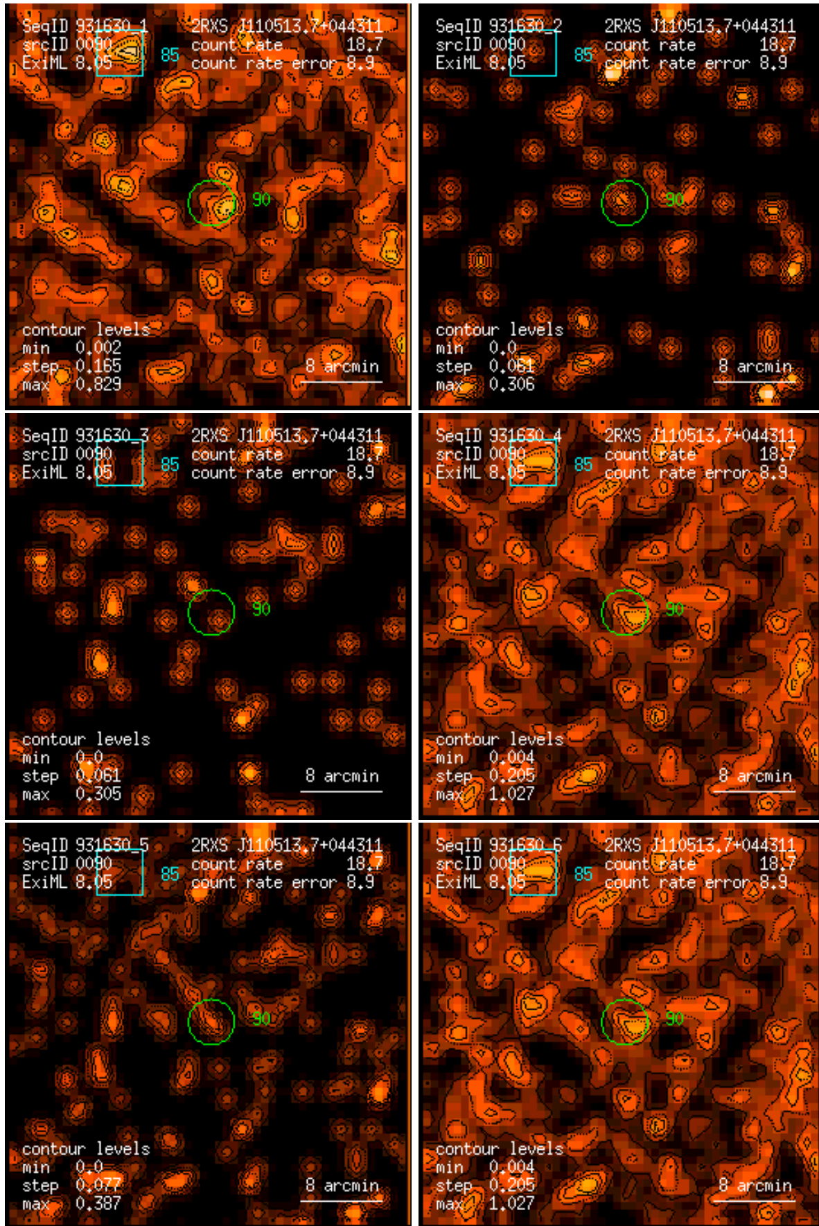
Figure 90: RASS 931630: detection 0090: band rate images, Gaussian filter: (1) PSPC channels 11 – 41, (2) 52 – 90, (3) 91 – 201, (4) 11 – 235, (5) 52 – 201, (6) 11 – 201. Broad band rates in counts/ks. Band rate contour levels in counts/ks/arcmin 2 .
