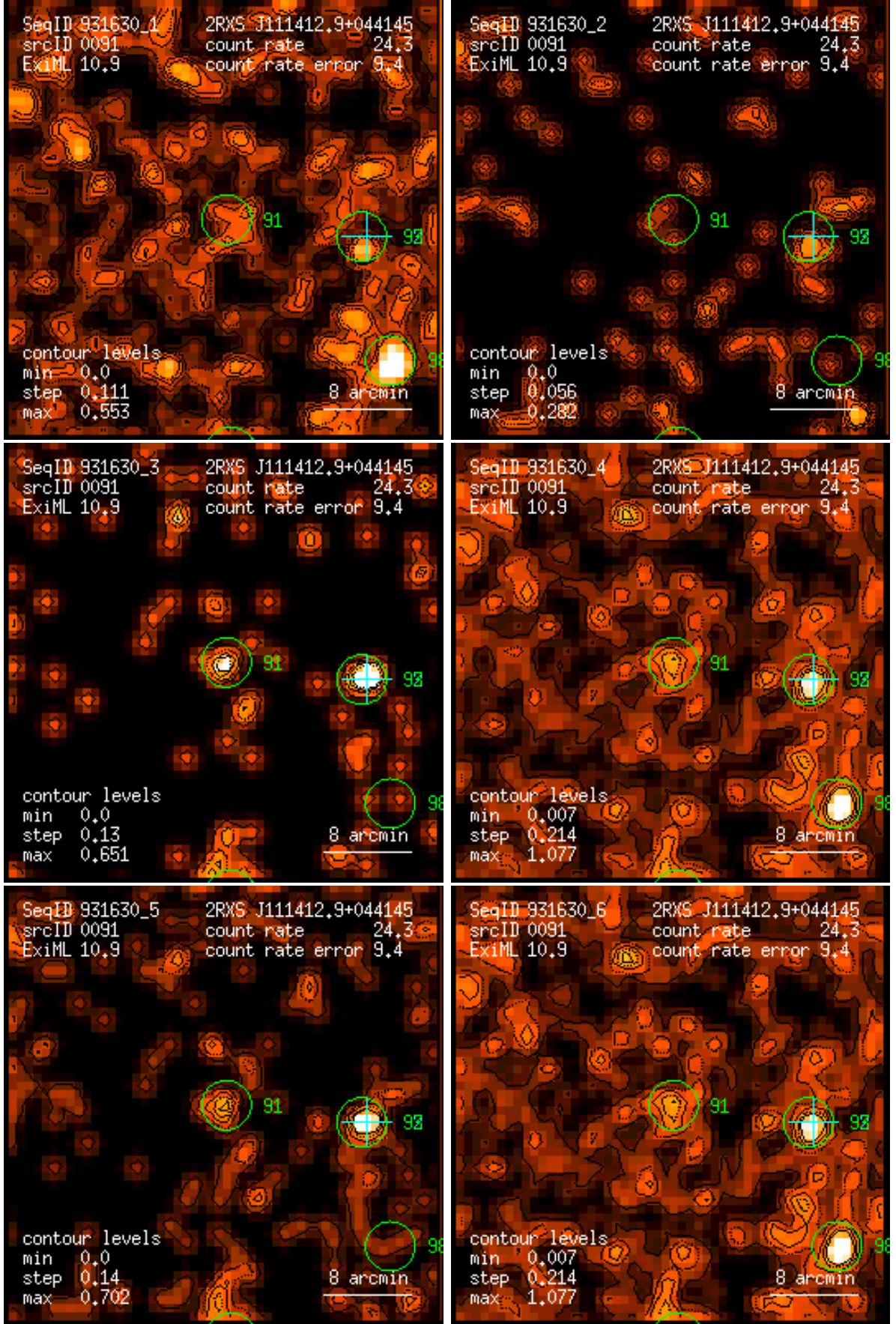
Figure 91: RASS 931630: detection 0091: band rate images, Gaussian filter: (1) PSPC channels 11 – 41, (2) 52 – 90, (3) 91 – 201, (4) 11 – 235, (5) 52 – 201, (6) 11 – 201. Broad band rates in counts/ks. Band rate contour levels in counts/ks/arcmin 2 .
