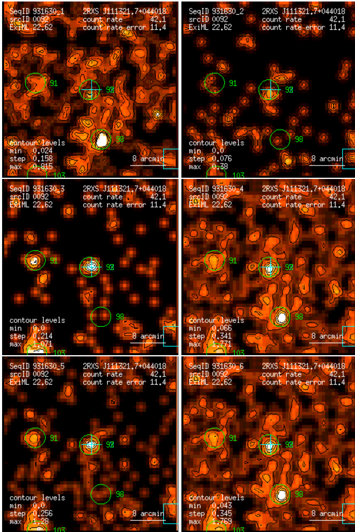
Figure 92: RASS 931630: detection 0092: band rate images, Gaussian filter: (1) PSPC channels 11 – 41, (2) 52 – 90, (3) 91 – 201, (4) 11 – 235, (5) 52 – 201, (6) 11 – 201. Broad band rates in counts/ks. Band rate contour levels in counts/ks/arcmin 2 .
