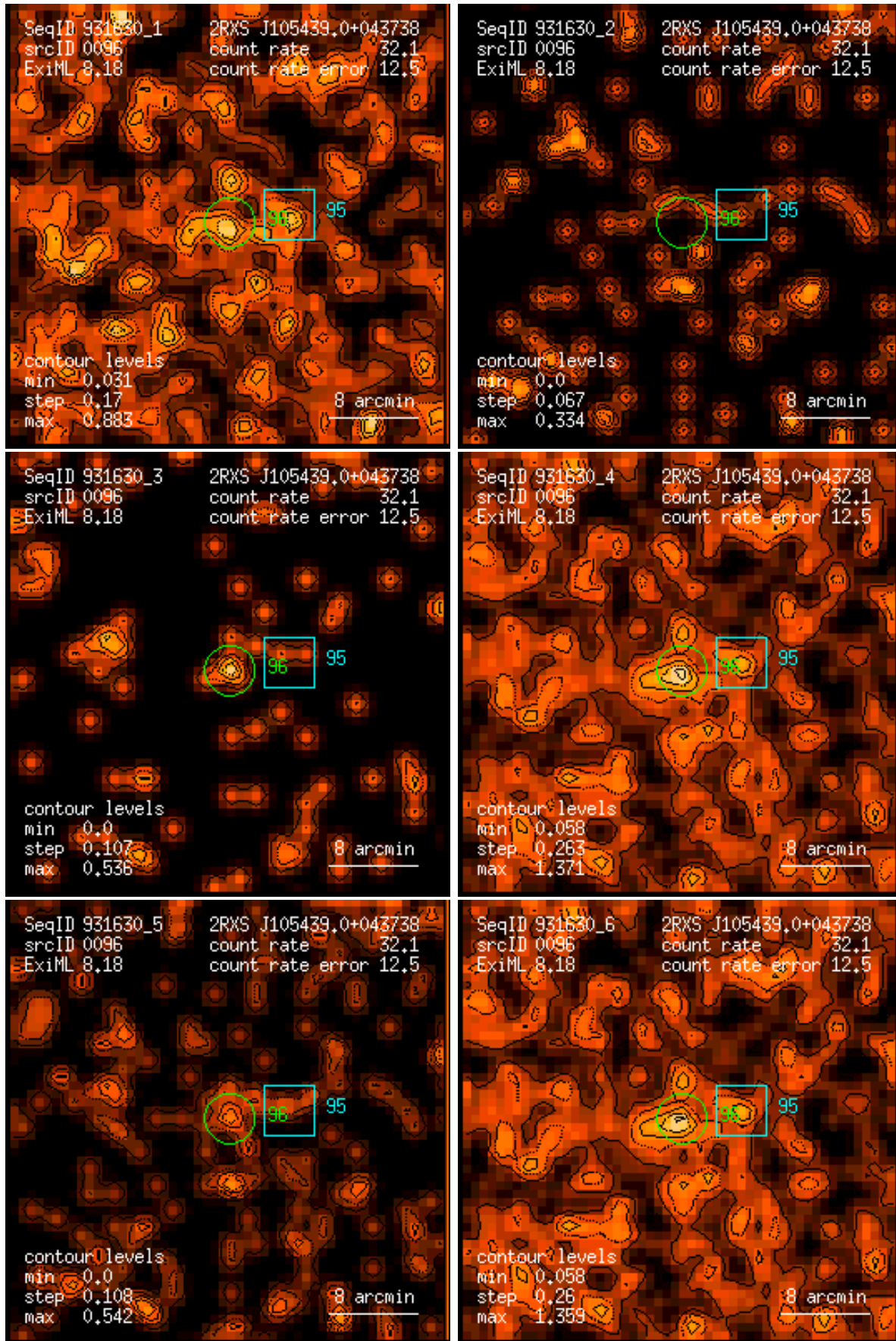
Figure 96: RASS 931630: detection 0096: band rate images, Gaussian filter: (1) PSPC channels 11 – 41, (2) 52 – 90, (3) 91 – 201, (4) 11 – 235, (5) 52 – 201, (6) 11 – 201. Broad band rates in counts/ks. Band rate contour levels in counts/ks/arcmin 2 .
