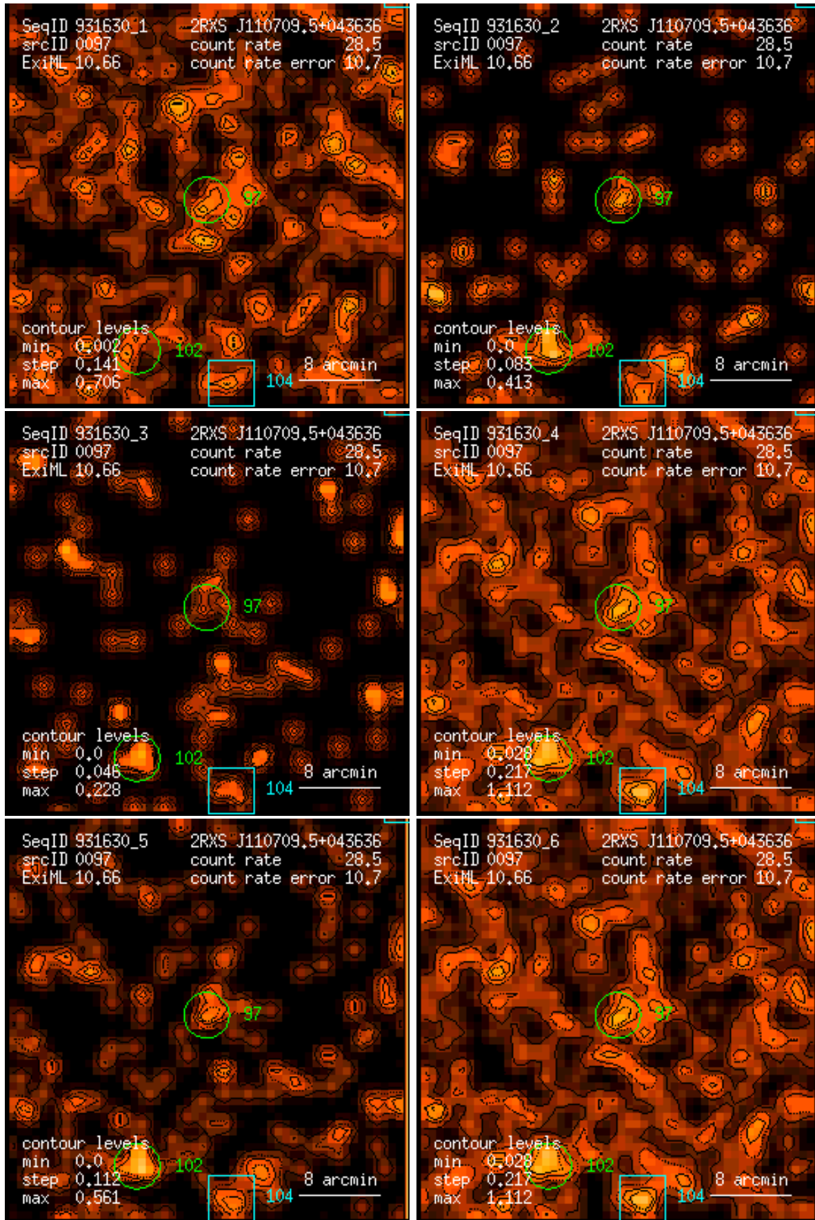
Figure 97: RASS 931630: detection 0097: band rate images, Gaussian filter: (1) PSPC channels 11 – 41, (2) 52 – 90, (3) 91 – 201, (4) 11 – 235, (5) 52 – 201, (6) 11 – 201. Broad band rates in counts/ks. Band rate contour levels in counts/ks/arcmin 2 .
