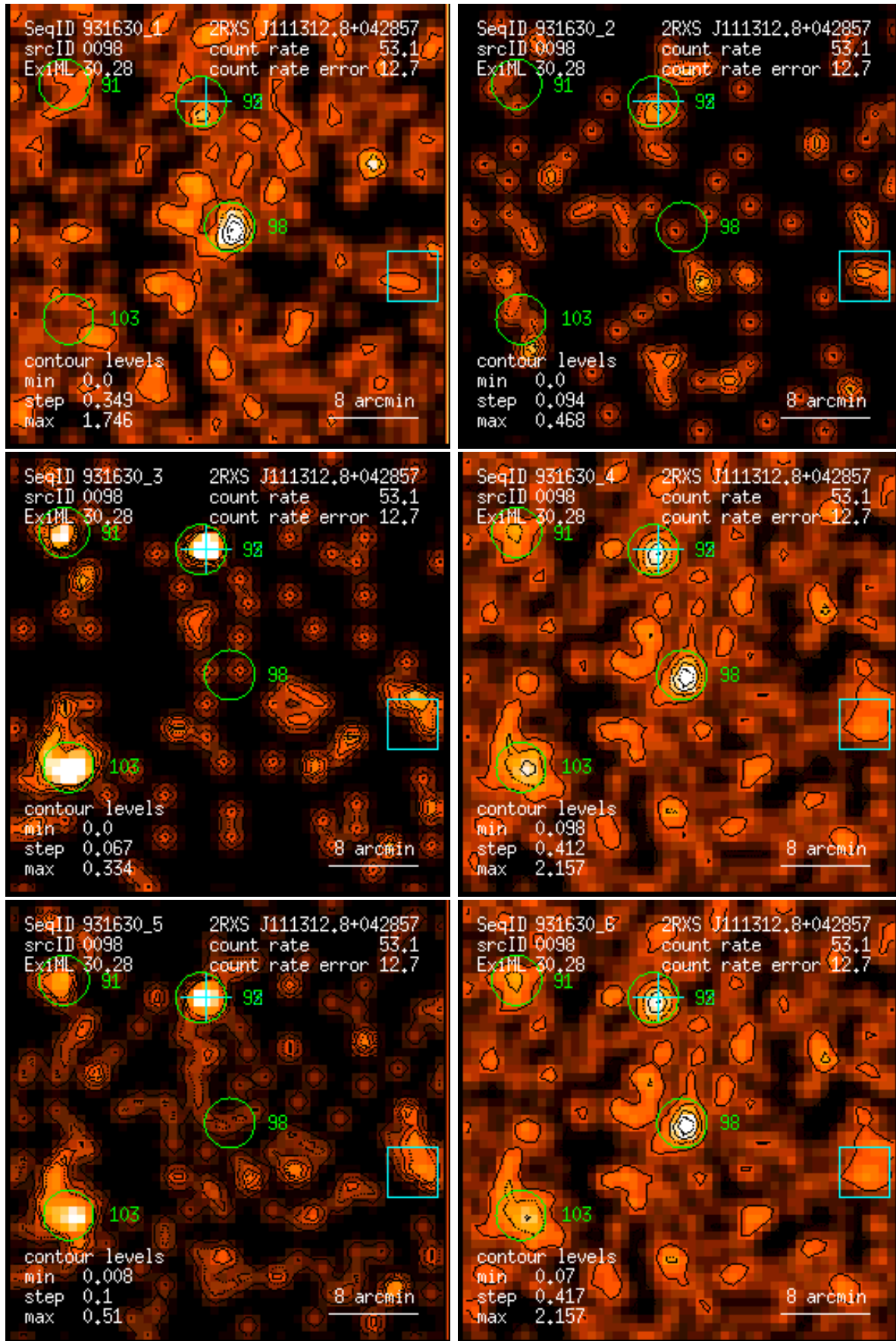
Figure 98: RASS 931630: detection 0098: band rate images, Gaussian filter: (1) PSPC channels 11 – 41, (2) 52 – 90, (3) 91 – 201, (4) 11 – 235, (5) 52 – 201, (6) 11 – 201. Broad band rates in counts/ks. Band rate contour levels in counts/ks/arcmin 2 .
