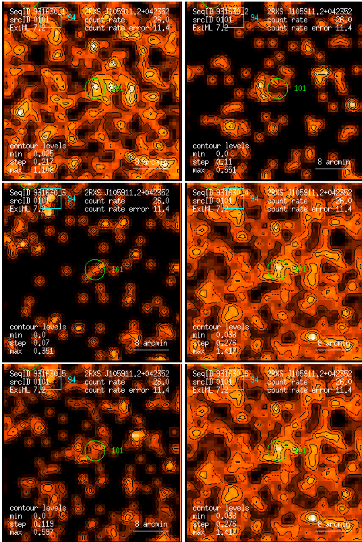
Figure 101: RASS 931630: detection 0101: band rate images, Gaussian filter: (1) PSPC channels 11 – 41, (2) 52 – 90, (3) 91 – 201, (4) 11 – 235, (5) 52 – 201, (6) 11 – 201. Broad band rates in counts/ks. Band rate contour levels in counts/ks/arcmin 2 .
