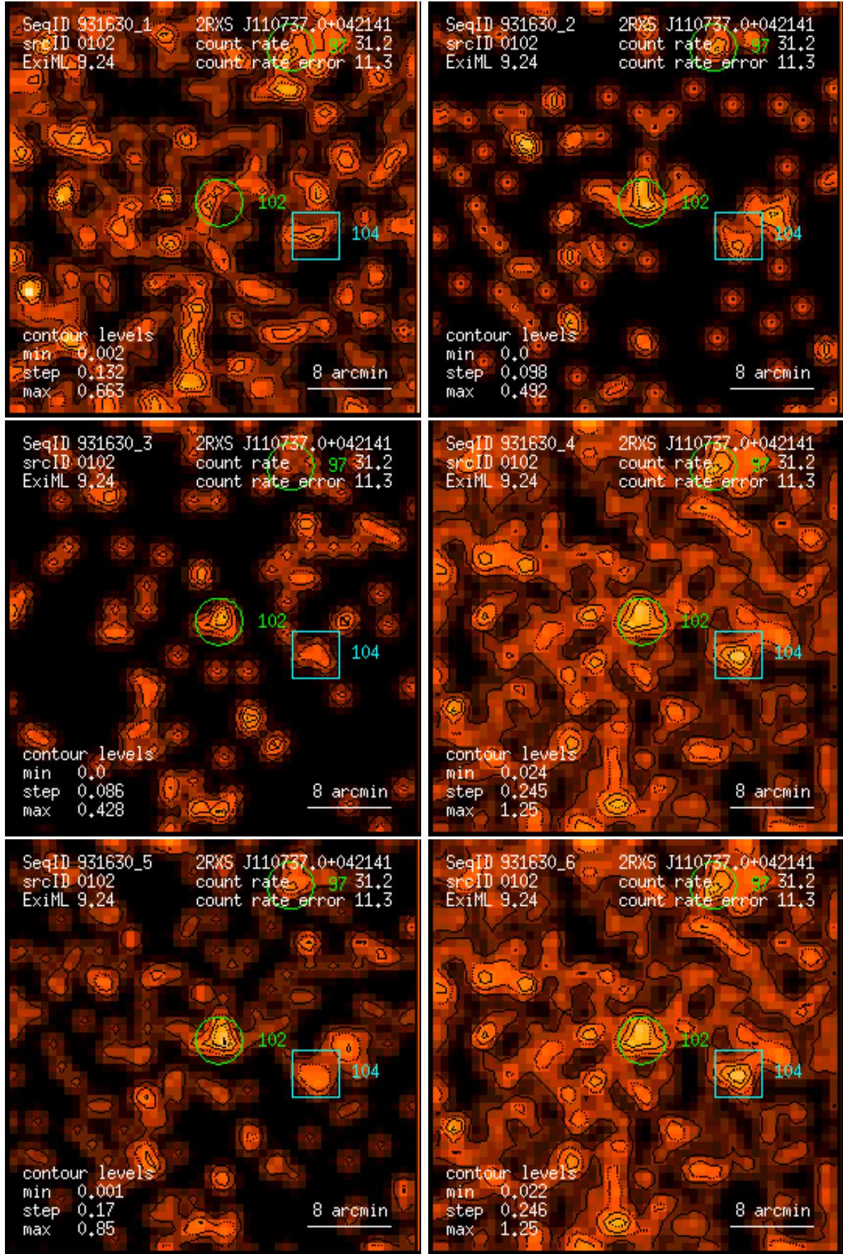
Figure 102: RASS 931630: detection 0102: band rate images, Gaussian filter: (1) PSPC channels 11 – 41, (2) 52 – 90, (3) 91 – 201, (4) 11 – 235, (5) 52 – 201, (6) 11 – 201. Broad band rates in counts/ks. Band rate contour levels in counts/ks/arcmin 2 .
