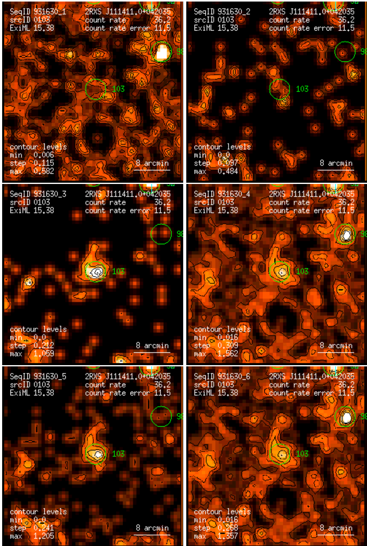
Figure 103: RASS 931630: detection 0103: band rate images, Gaussian filter: (1) PSPC channels 11 – 41, (2) 52 – 90, (3) 91 – 201, (4) 11 – 235, (5) 52 – 201, (6) 11 – 201. Broad band rates in counts/ks. Band rate contour levels in counts/ks/arcmin 2 .
