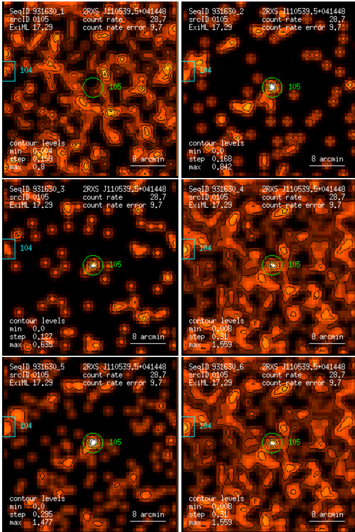
Figure 105: RASS 931630: detection 0105: band rate images, Gaussian filter: (1) PSPC channels 11 – 41, (2) 52 – 90, (3) 91 – 201, (4) 11 – 235, (5) 52 – 201, (6) 11 – 201. Broad band rates in counts/ks. Band rate contour levels in counts/ks/arcmin 2 .
