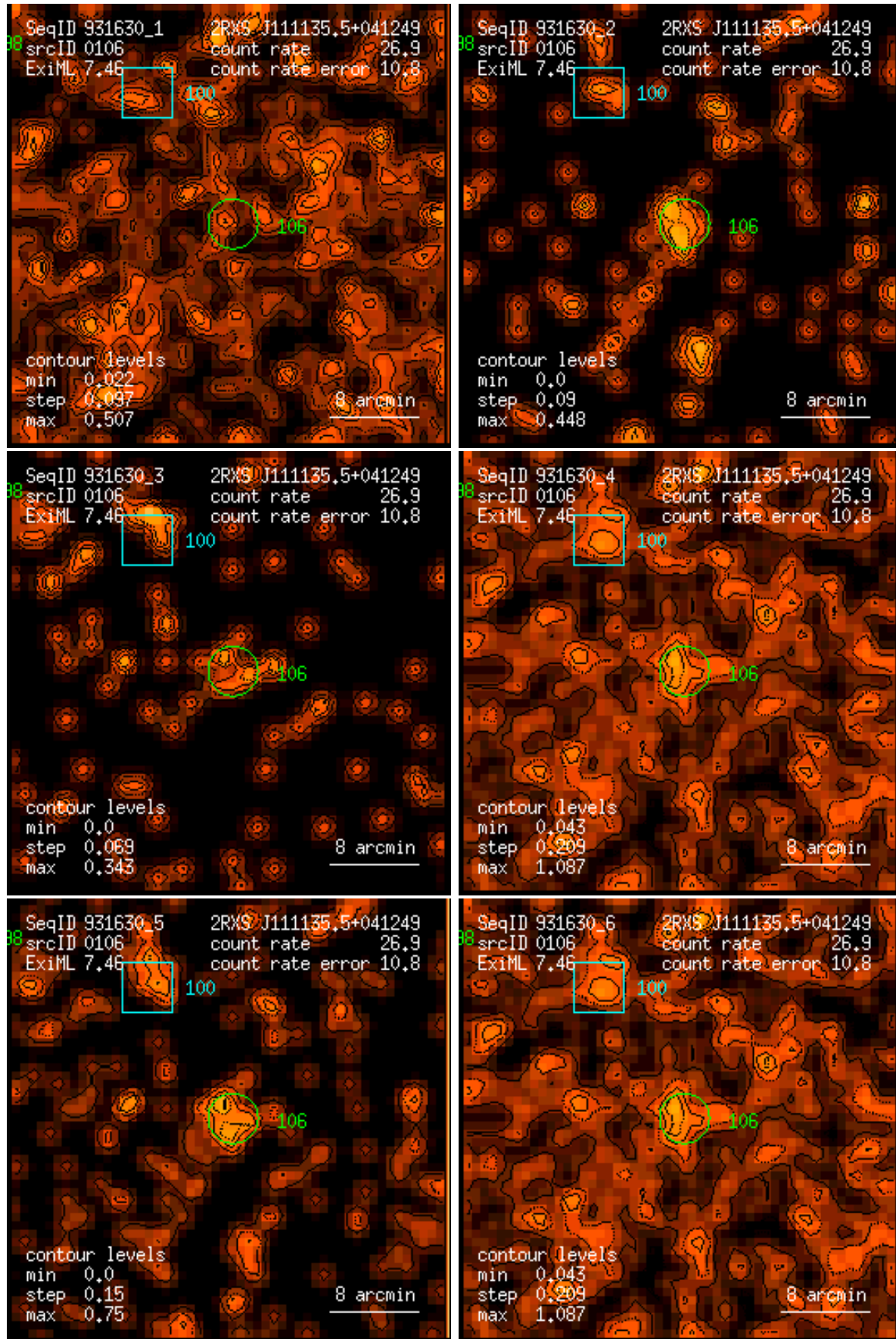
Figure 106: RASS 931630: detection 0106: band rate images, Gaussian filter: (1) PSPC channels 11 – 41, (2) 52 – 90, (3) 91 – 201, (4) 11 – 235, (5) 52 – 201, (6) 11 – 201. Broad band rates in counts/ks. Band rate contour levels in counts/ks/arcmin 2 .
